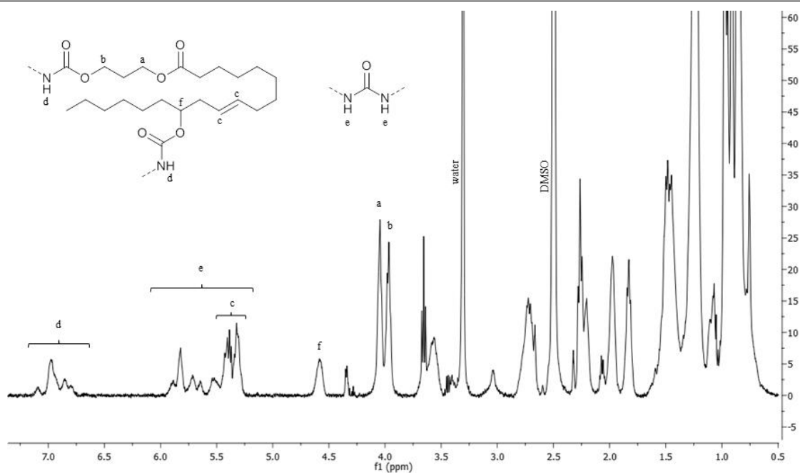
Fig. 2: ^1\text{H} NMR in deuterated DMSO of lyophilized polymer latex with partial assignment. ( RicPmE and IPDI were used as monomers, with 3.5 CMC of SDS. No hydrophobic agent was added. DBTDL concentration was 0.4wt% of the organic phase.)
