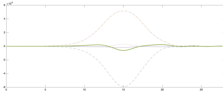
FIGURE 12. Decomposition of the vertical force F_{\text{vert}} (thick solid line) exerted on the structure, as in (74). Damping-excitation force F_{\text{D+E}} (dash-dot), restoring force F_{\text{restor}} (dash), force due to added mass F_{\text{added}} (dots) and nonlinear corrections F_{\text{NL}} (solid).
