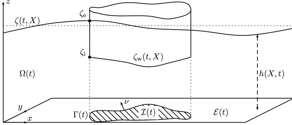
FIGURE 2. The case of vertical walls
