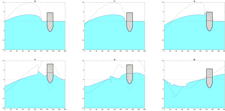
FIGURE 9. A wave arriving on a freely floating structure (nonlinear shallow water model). Surface elevation (full), initial condition (dots) and rescaled discharge (dash). The horizontal line on the structure marks the contact line at the equilibrium.
