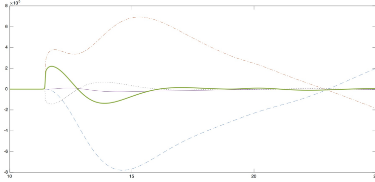
FIGURE 10. Decomposition of the vertical force F_{\text{vert}} (thick solid line) exerted on the structure, as in (74). Damping-excitation force F_{\text{D+E}} (dash-dot), restoring force F_{\text{restor}} (dash), force due to added mass F_{\text{added}} (dots) and nonlinear corrections F_{\text{NL}} (solid).
