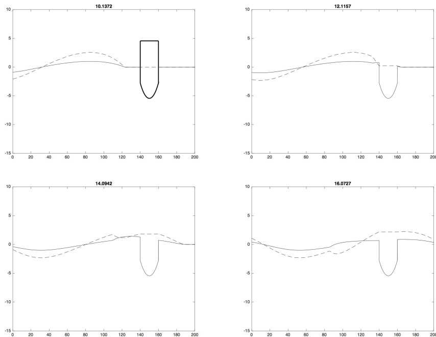
FIGURE 6. A wave arriving on a fixed floating structure. Surface elevation (full) and discharge (divided by a rescaling factor 5, dash).
