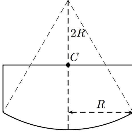
FIGURE 5. Shape of the floating structure
