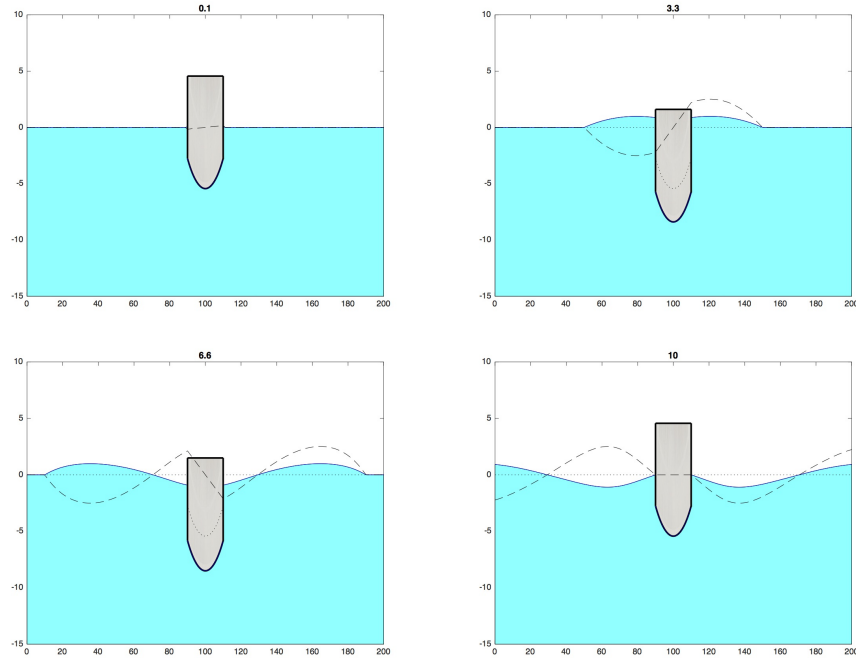
FIGURE 7. A solid in forced vertical motion. Surface elevation (full) and discharge (divided by a rescaling factor 5, dash), initial position (dots).
