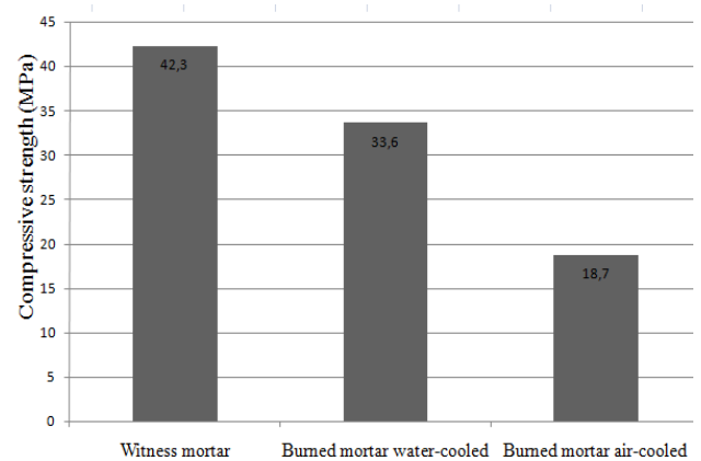
Figure 7a: Compressive strength
