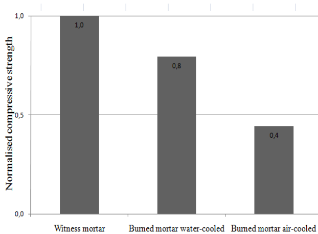
Figure 7b: Compressive strength: values normalized to the strength of witness mortar
