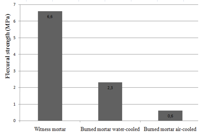
Figure 6a : Flexural strength
