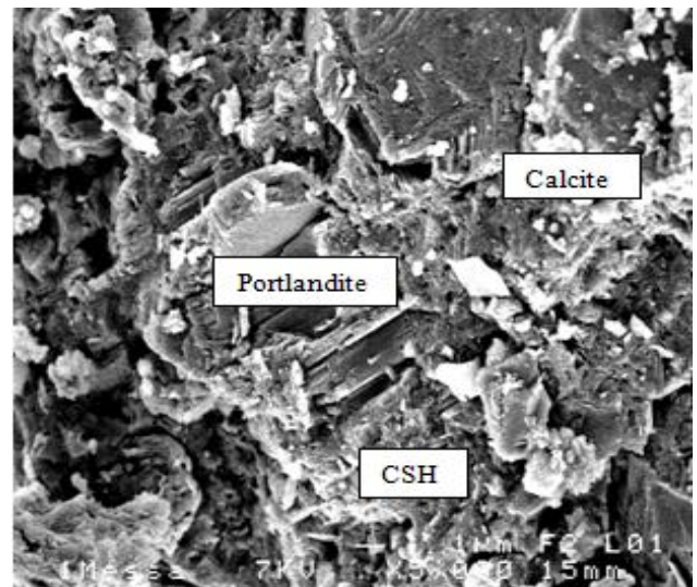
Figure 9: SEM observation of witness cement
