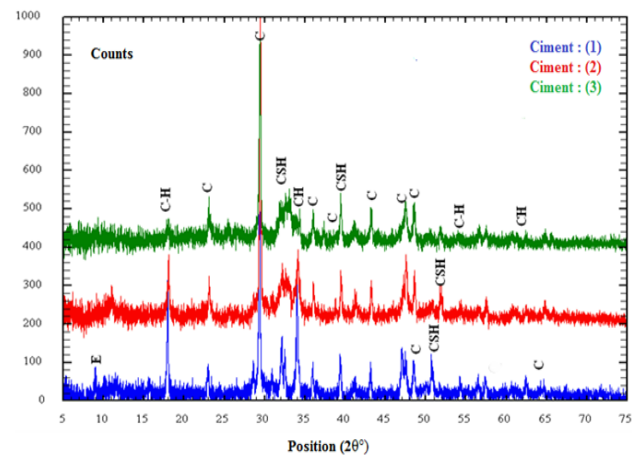
Figure 8: X-ray diffraction of cement pastes 1, 2 and 3
