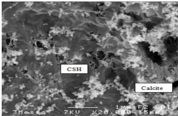
Figure 10: SEM observation of burned cement
