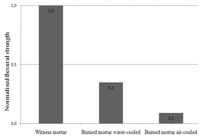
Figure 6b: Flexural strength: values normalized to the strength of witness mortar
