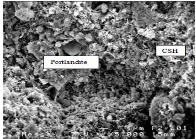
Figure 11: SEM observation of burned cement soaked in water
