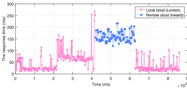
Fig. 5. The measured response time from our experiment, measured for each web request as time elapses; the different colours represent the different clouds where the requests are allocated and processed.
