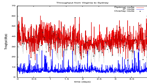
Fig. 7. Throughput (Mbps) measured from Virginia (USA) to Sydney (Australia) over 4 consecutive days.
