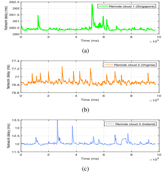
Fig. 4. The weighted average network delay over time on the connections to the three remote clouds; it is derived from the measurement of the round-trip delay and loss via ping.
