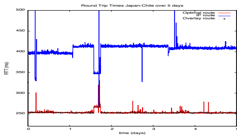
Fig. 6. RTD in milliseconds measured for the Japan-Chile connection in an experiment lasting 5 successive days.
