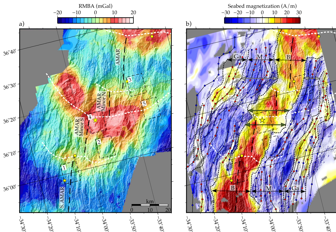
Figure 4. (a) Residual Mantle Bouguer Anomaly (RMBA) with superimposed terrain illumination calculated from the bathymetry grid. (b) Seabed magnetization calculated from inversion of the magnetic anomaly assuming a constant thickness source layer (500 m). Again the terrain illumination is superimposed on the color map. Dashed black curves mark the magnetic reversals between major magnetic chrons (B=Brunhes, M=Matuyama, Ga=Gauss). Normal polarity chrons are marked by black lines with red dots. Reverse polarity chrons are marked by black lines with blue dots. The magnetic chrons were picked from laterally continuous local maxima and minima in the magnetization map with aid from the geomagnetic timescale of Gee and Kent [2007]. In both plots, the map projection is rotated to align the horizontal with the spreading direction. A dashed black line marks the ridge axis. Dashed white lines mark the boundaries between ridge segments. The Rainbow hydrothermal field is marked by a yellow star. Other identified hydrothermal sites and plumes are marked by yellow circles. Areas shown in Figure 5 are marked by dashed boxes.
