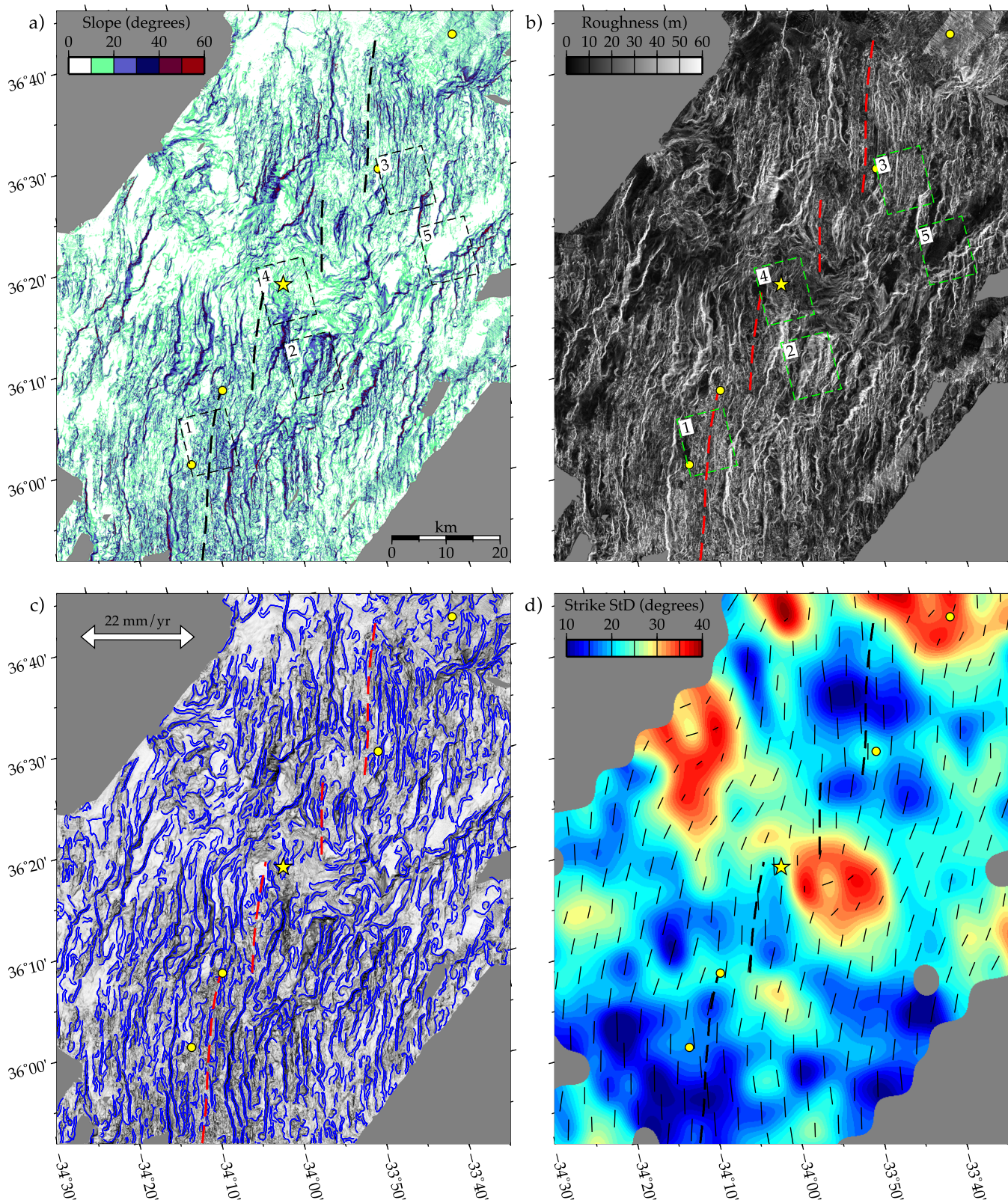
Figure 2. Morphometric maps calculated from the multibeam bathymetry grid. In all plots the projection is rotated to align the horizontal with the spreading direction. (a) Slope gradient. (b) Roughness. (c) Seabed lineaments drawn from the slope map using an edge detection algorithm. The slope gradient is plotted for reference in the background with a gray color scale. (d) Standard deviation of the lineament strike within 0.1^\circ \times 0.1^\circ cells. This map highlights areas where the seabed fabric lacks organized alignment. Superimposed black bars show local average of lineament direction. A thick dashed line marks the ridge axis. The Rainbow hydrothermal field is marked by a yellow star. Other identified hydrothermal sites and plumes are marked by yellow circles. Numbered dashed boxes correspond to areas shown in Figure 5.
