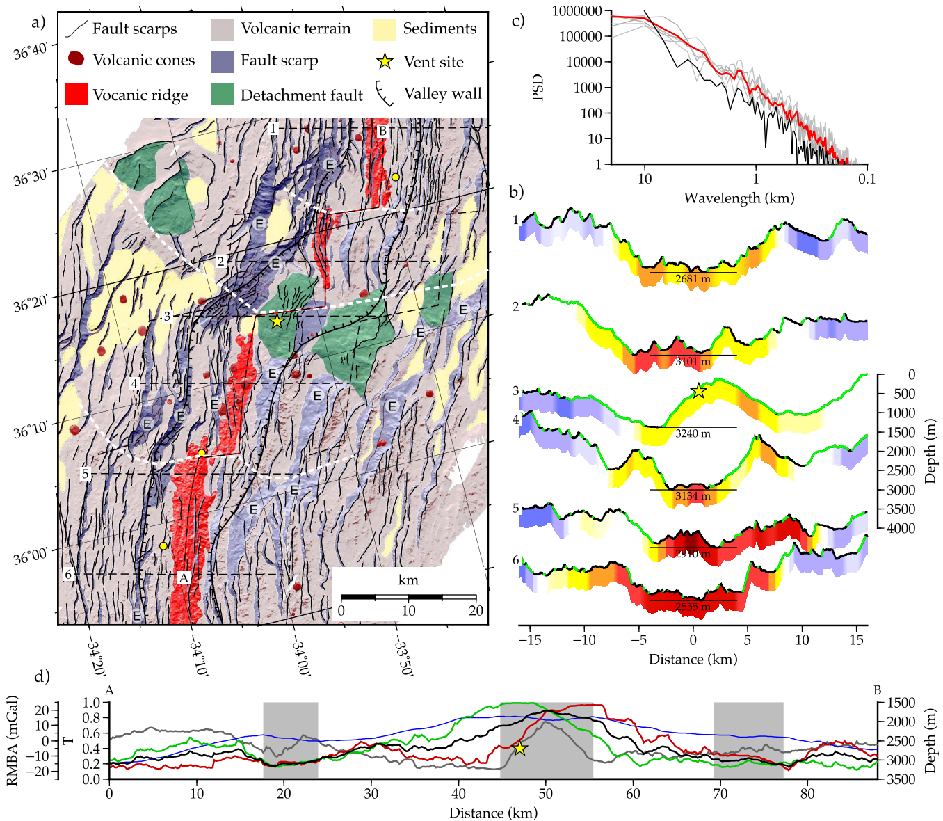
Figure 6. (a) Map interpretation of the Rainbow area. The map projection is rotated to align the horizontal with the spreading direction. Major mode E faults are marked (E). The profiles shown in Figures 6b and 6d are marked by black dashed lines. Dashed white lines mark the boundaries between ridge segments. (b) Across axis profiles of bathymetry. Green sections correspond to exposed fault surfaces identified in Figure 6a. The seabed magnetization extracted from the grid shown in Figure 4b is drawn beneath each profile (same color scale). (c) Power spectral density of the profiles shown in Figure 6b. A thicker black line marks the spectrum of the profile crossing the Rainbow massif, which shows a reduced short wavenumber component. The average of all other profiles is drawn in red. (d) Along-axis profile (AB) of bathymetry (gray), RMBA (blue) and tectonic strain, T , (black). T is calculated over profiles extracted every 200 m along AB and extending 16 km off-axis in either direction parallel to the far-field spreading vector and to the profiles shown in (b). Red curve shows T calculated on W flank only; green curve shows T for E flank only.
