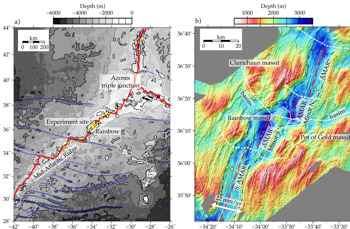
Figure 1. (a) Bathymetric map of the Mid-Atlantic Ridge showing the experiment site, the ridge axis (red) and major fracture zones (blue). (b) Bathymetric map of the survey area. The Rainbow massif and other massifs interpreted as remnants of core complexes are outlined in white. The ridge axis is marked with a red dashed line. Its location was determined from the analysis of the bathymetry and potential field data. Note the three ridge offsets. A dashed/dotted line marks the axial valley walls. Dashed white lines mark the boundaries between ridge segments. The rainbow hydrothermal field is marked with a yellow star. The location of other identified hydrothermal sites or plumes are marked with yellow circles (InterRidge Vents Database 3.2, http://vents-data.interridge.org/ ). A white arrow marks the spreading vector direction.
