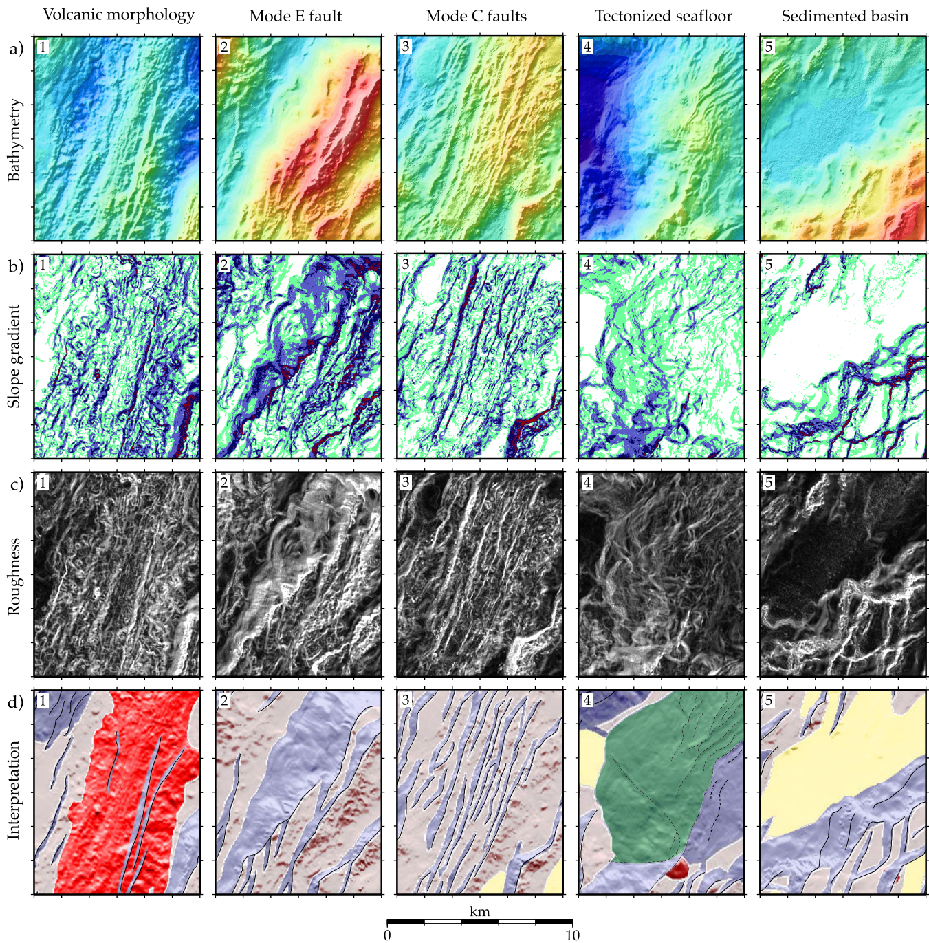
Figure 5. Detail of morphological features. (a) Elevation with terrain illumination from the NW, color scale as in Figure 1a. (b) Slope gradient, color scale as in Figure 2a. (c) Roughness, color scale as in Figure 2b. (d) Geological interpretation, color scale as in Figure 6a. Column 1: Example of volcanic morphology on the axial volcanic ridge; column 2: large mode E fault and back-tilted volcanics; column 3: mode C faults and volcanic terrain; column 4: tectonized seafloor including the Rainbow massif; column 5: sediment-filled basin and interlinked faults.
