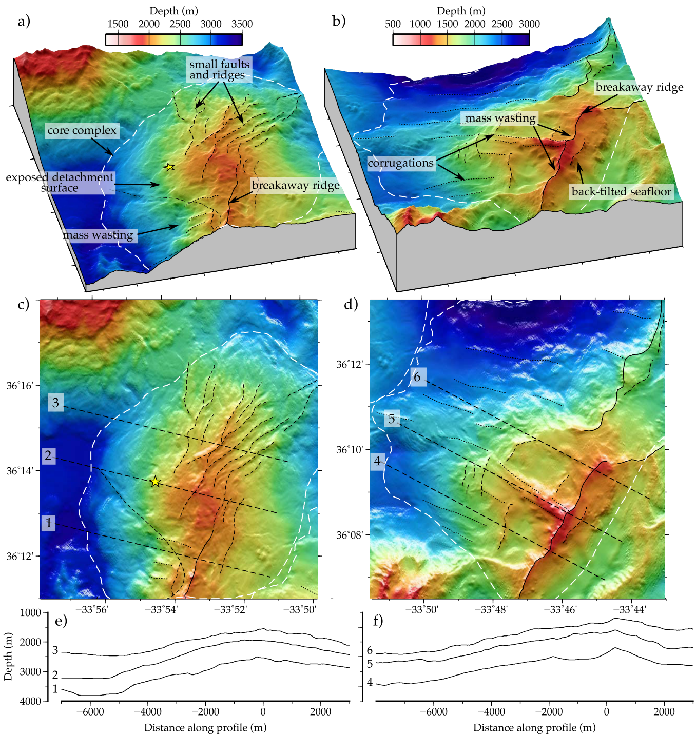
Figure 7. Detailed bathymetric maps of the Rainbow and Pot of Gold massifs/OCCs. (left) Rainbow massif; (right): Pot of Gold massif. (a, b) Three-dimensional isometric views. (c, d) Illuminated bathymetry and location of profiles shown in Figures 7e and 7f. The yellow star marks the location of the RHF. White dashed lines mark the extent of the OCCs, including the fossil detachment fault surfaces and back-tilted seafloor. (e, f) Cross sections through the OCCs showing the geometry of the flexural dome and back-tilted seabed.
