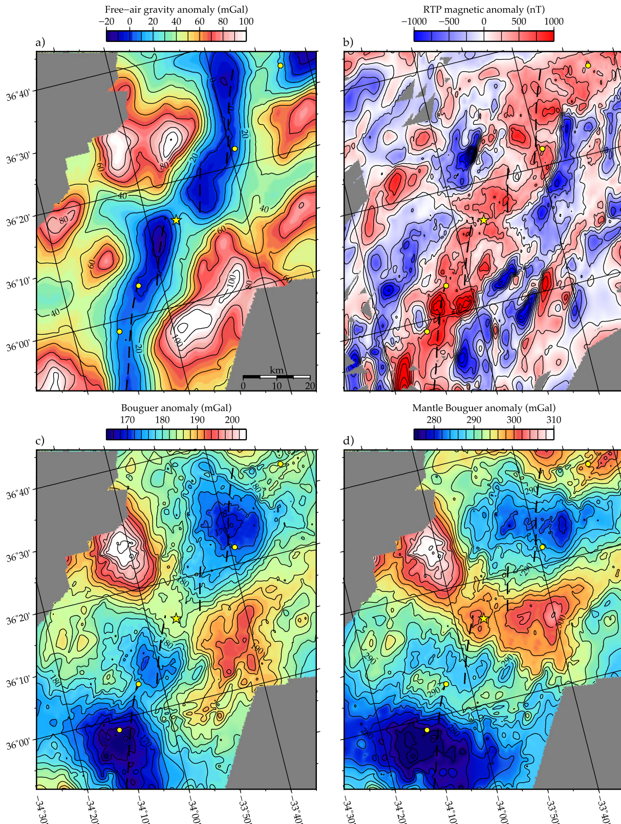
Figure 3. Analysis of the potential field data. (a) Free-air gravity anomaly at the sea surface calculated from shipboard gravity data. (b) Reduced-to-pole magnetic anomaly. (c) Bouguer gravity anomaly assuming a crustal density of 2700 \text{ kg/m}^3 . (d) Mantle Bouguer anomaly assuming a 400 \text{ kg/m}^3 density contrast at 4.5 km depth below the seabed. In all plots the map projection is rotated to align the horizontal with the spreading direction. A dashed black line marks the ridge axis. The Rainbow hydrothermal field is marked by a yellow star. Other identified hydrothermal sites and plumes are marked by yellow circles.
