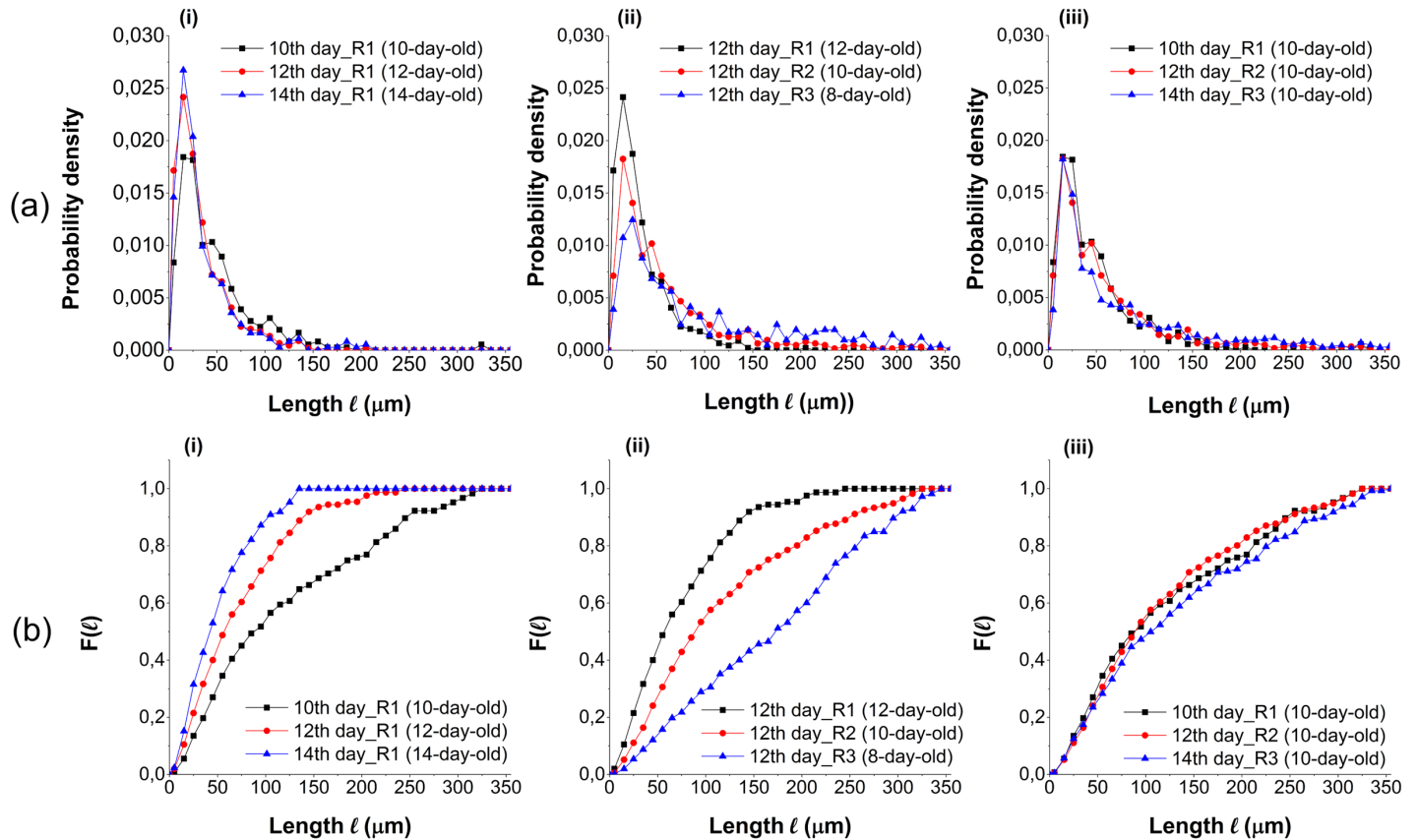
Fig 7. (a) Branching length distribution and (b) the corresponding weighted cumulative distribution F(\ell) . The different graphs depict (i) the same region on different observation days, (ii) the different regions on the same observation day, (iii) the distributions of different regions on observation days selected to have the same hyphal age.
