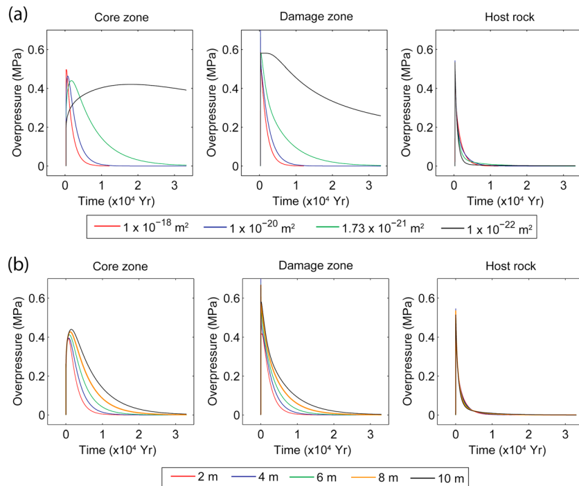
Figure 12. Sensitivity tests of the fault drained response illustrating the influence of change in (a) permeability and (b) width of damage zone on the fluid overpressures from the core through the damage zone to the host rock.
