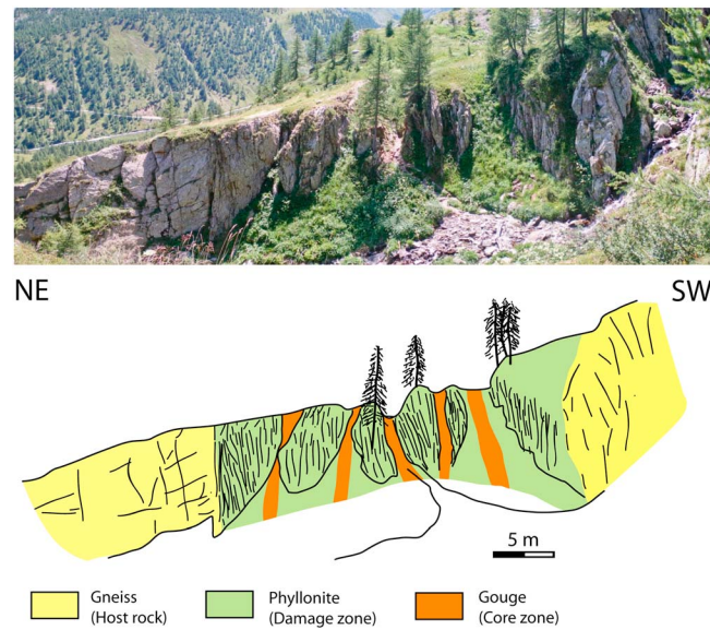
Figure 2. Photograph and corresponding sketch of the studied outcrop. The fault zone shows anastomosed core zones surrounded by damage zones with a pluri-decamic total width. The core zones are made of centimetric to metric phyllosilicate-rich gouge layers. The damage zones are composed of pluri-metric phyllonitic rocks derived from mylonite. The host rock is composed of gneiss.
