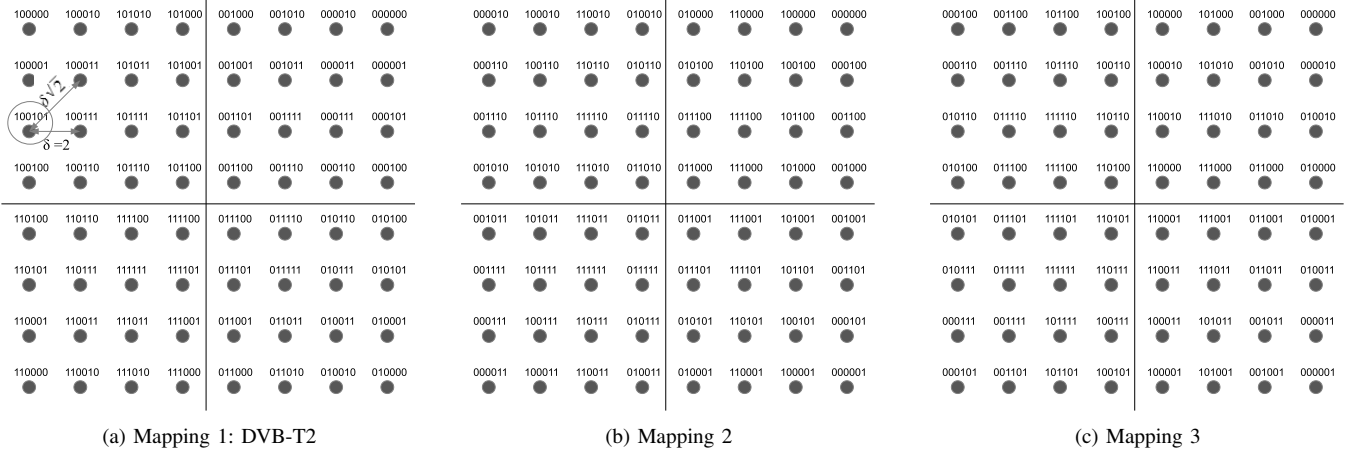
Fig. 1: Gray mappings for coded modulations \mathcal{C}_1 , \mathcal{C}_2 and \mathcal{C}_3
