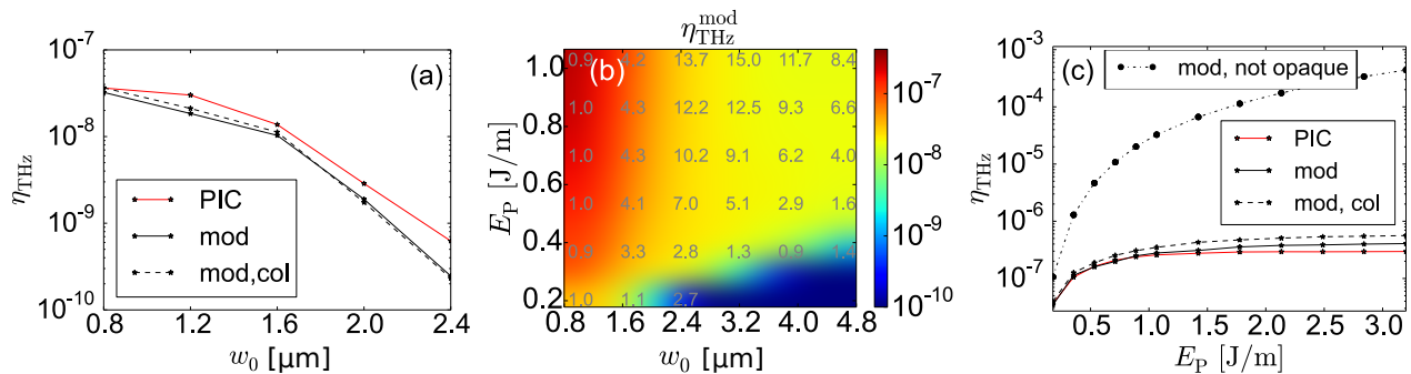
FIG. 10. Scaling of the conversion efficiency \eta_{\text{THz}} with focal spot-size and pulse energy, for fixed laser wavelength \lambda_L = 0.8 \mu\text{m} , pulse duration t_0 = 50 \text{ fs} and argon gas density n_a = 3 \times 10^{19} \text{ cm}^{-3} . In (a), PIC results (solid red line) and the simplified model (solid black line) for a laser pulse energy of E_p = 0.18 \text{ J/m} are shown. The black dashed line shows model results accounting for collisions. In (b), the model is evaluated in the (w_0, E_p) -plane. Ratios of PIC and model conversion efficiencies are indicated in gray. In (c), \eta_{\text{THz}} as a function of the pulse energy is shown for tight focusing ( w_0 = 0.8 \mu\text{m} ). Results from PIC simulations (solid red line) and the simplified model with and without collisions (dashed and solid black line, resp.) are in good agreement. The black dashed-dotted line shows model results when the opaqueness of the plasma is ignored (see text).
