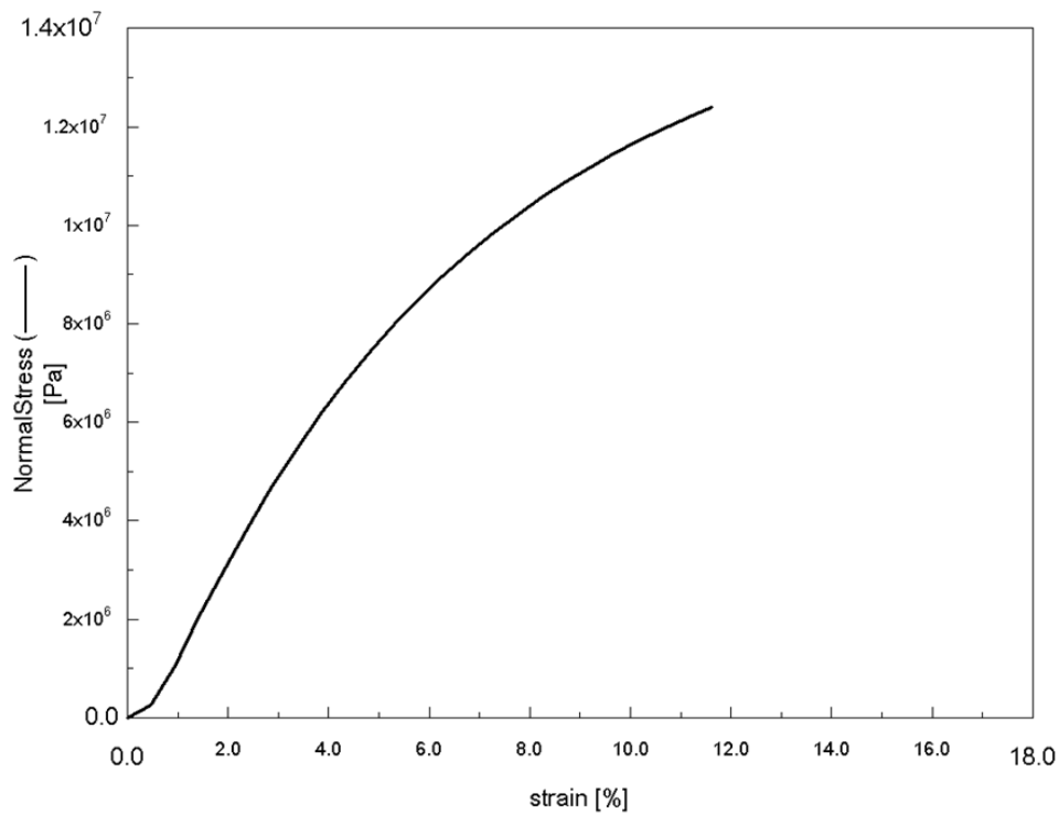
Figure S3. stress-strain curve of PEA – 10\text{mm}\cdot\text{min}^{-1} .
