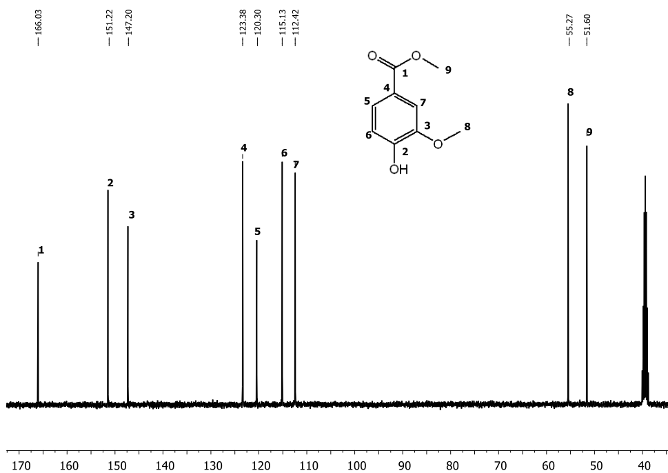
Figure S102: ^{13}\text{C} NMR spectrum of methyl vanillate in DMSO, at room temperature.
