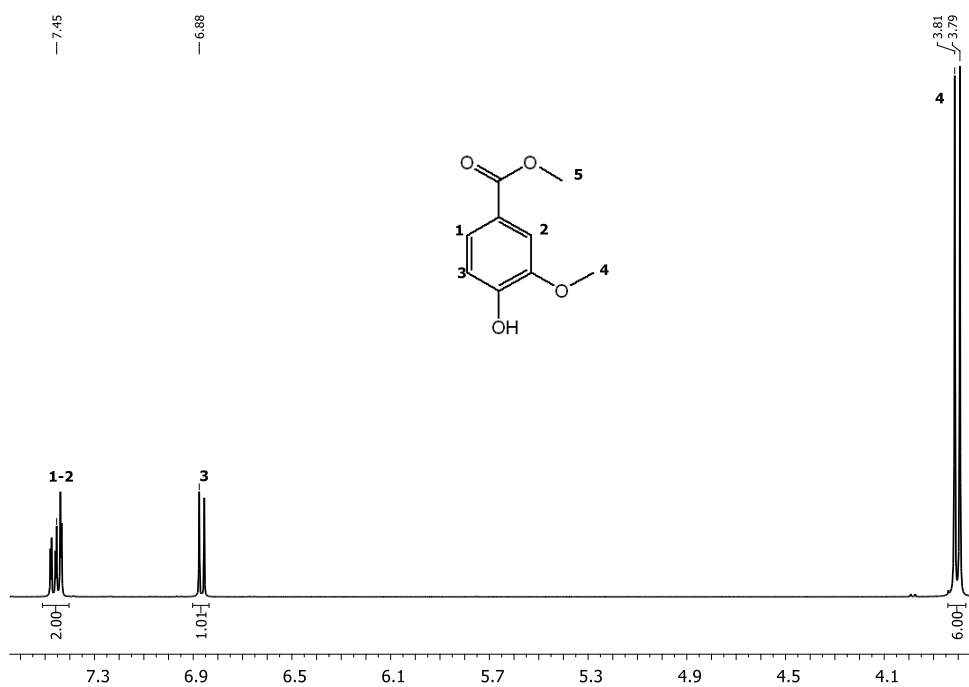
Figure S91: ^1\text{H} NMR spectrum of methyl vanillate in DMSO, at room temperature.
