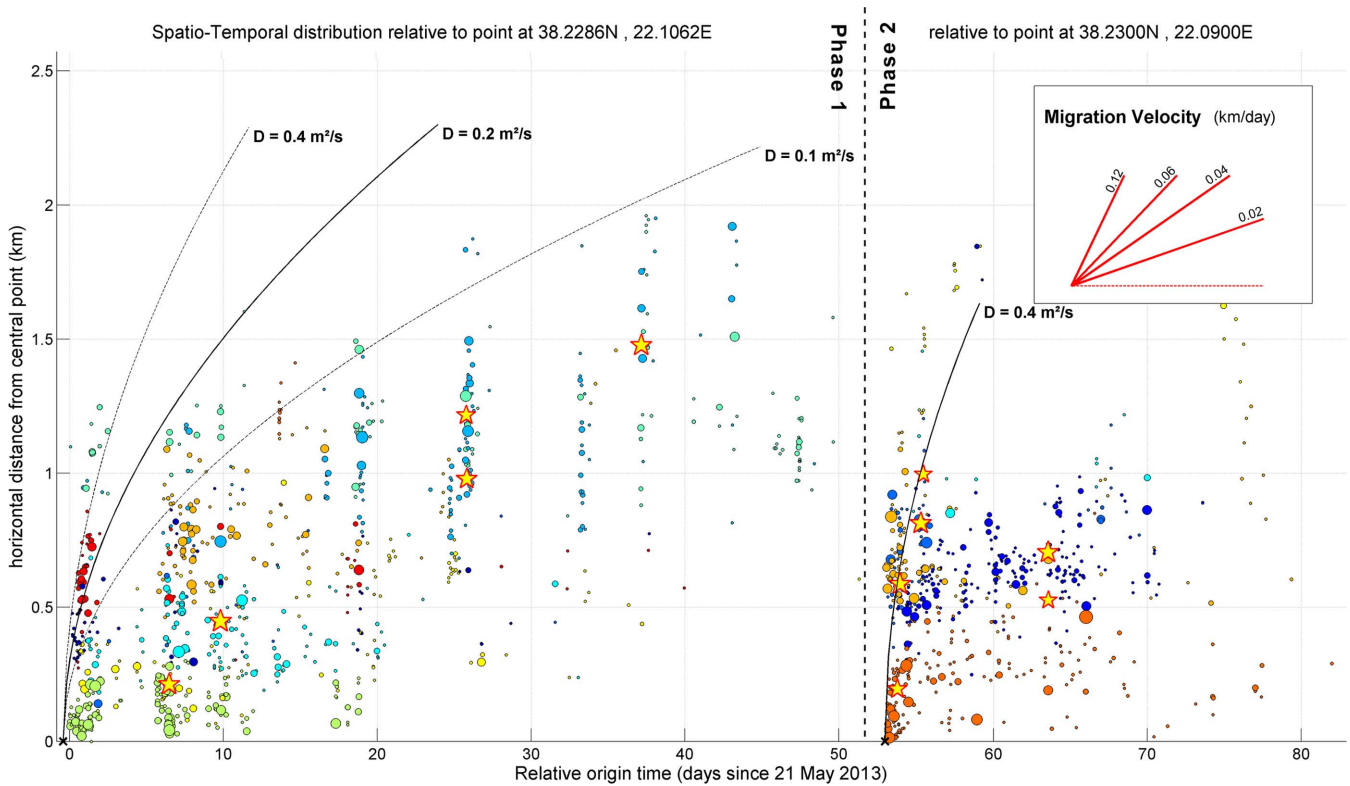
Figure 18. Spatiotemporal distribution of epicentres relative to possible fluid intrusion sources located at [38.2286°N, 22.1062°E] (left, phase 1, eastern part) and [38.2300°N, 22.0900°E] (right, phase 2, western part). Colours correspond to different spatial clusters. Parabolic theoretical curves of probable triggering fronts for hydraulic diffusivity values D = 0.4 \text{ m}^2 \text{ s}^{-1} , D = 0.2 \text{ m}^2 \text{ s}^{-1} and D = 0.1 \text{ m}^2 \text{ s}^{-1} are also displayed.
