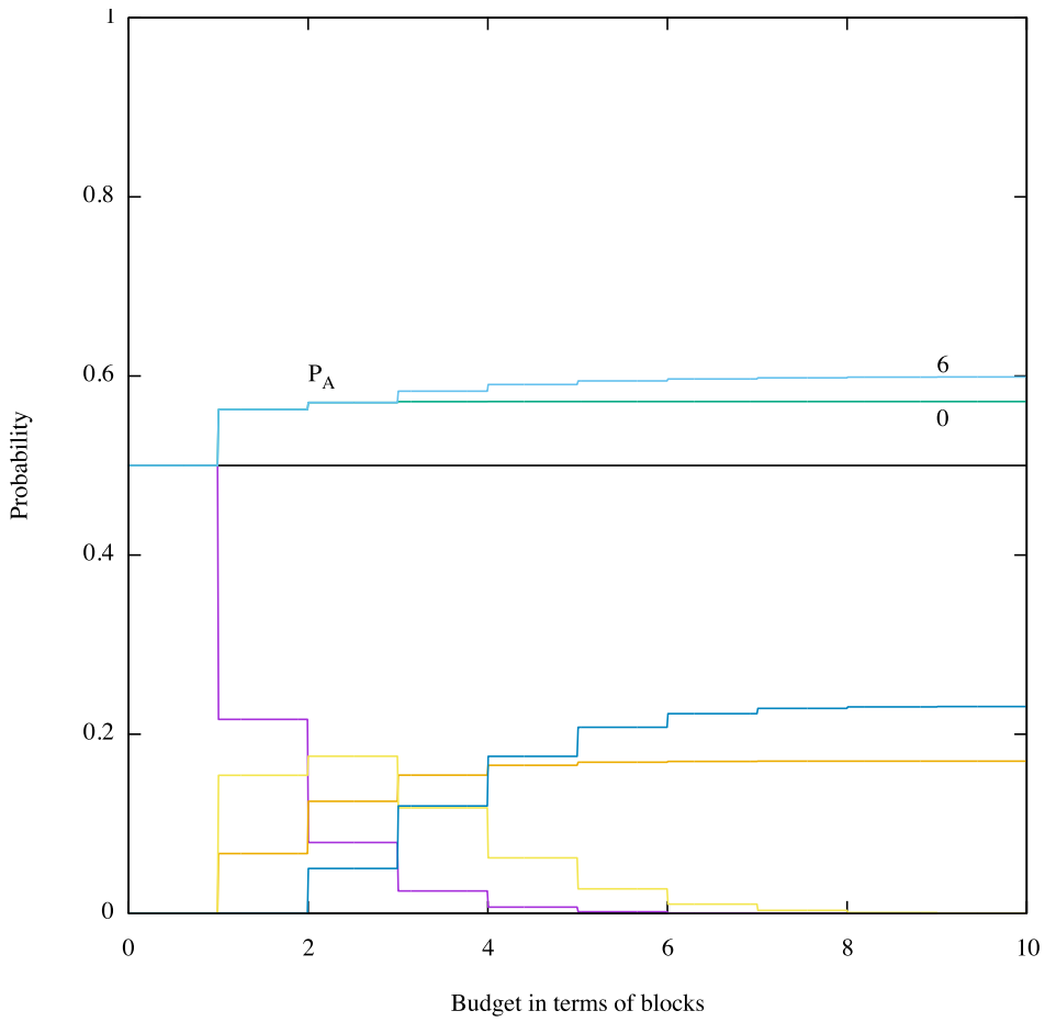
Fig. 6. Probabilities as functions of the budget (number of blocks that can be dropped), when \lambda = 1/4 and \mu = 1/2 . The two highest curves correspond to \mathcal{P}_{\mathcal{A}} in the delay-free case ( \Delta = 0 ) and when \Delta = 6 . The lowest curves are the four components that permit to compute \mathcal{P}_{\mathcal{A}} when \Delta = 6 : the purple curve corresponds to \Pr(f \wedge \mathbf{b} \wedge \sigma) , the orange one to \Pr(f \wedge \neg \mathbf{b} \wedge \sigma) , the blue one to \Pr(f \wedge \neg \mathbf{b} \wedge \neg \sigma) , and the yellow one to \Pr(f \wedge \mathbf{b} \wedge \neg \sigma) .
