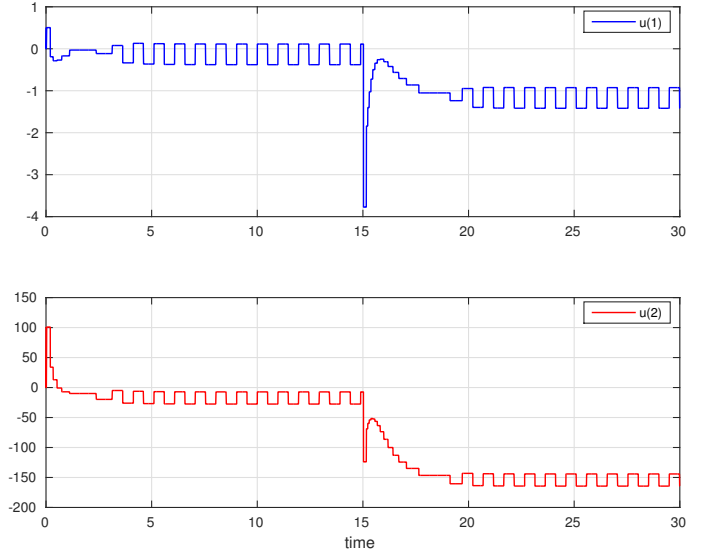
Fig. 5. The event-based control signal
