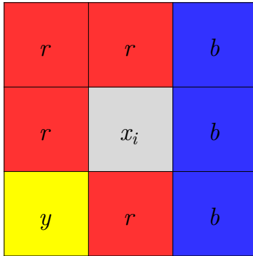
Figure .15: Examples of target neighborhoods for which detailed balance condition is not satisfied with the target value selection used within the MMA (step (2b.)): either with a target neighborhood equal to the Von Neumann or Moore neighborhood, the site value r has more chance to be selected than site values b or y .
