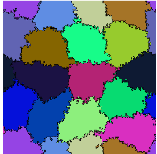
Figure 1: Cell fragmentation observed with the MMA at high temperature values: fragments of one or more lattice sites are surrounded by mismatched site values. Here each cell has a different color to highlight the presence of fragments.
