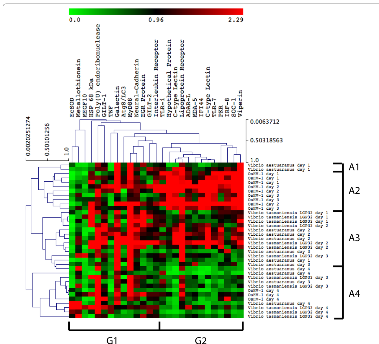
Figure 5 Heat map depicting the expression of immune genes of adult Crassostrea gigas infected with OsHV-1, Vibrio aestuarianus and V. tasmaniensis LGP32. The expression of each target gene was normalised to the transcript level of control groups (adults injected with sterile seawater) at each sampling time point (1, 2, 3 and 4 days post-injection). Adult oysters in the early stages of OsHV-1 infection (A2) cluster separately to adult oysters in the early (A3) and late (A4) stages of Vibrio infection. Hierarchical clustering did not reveal a distinction in the transcriptional response of adult C. gigas infected with V. aestuarianus or V. tasmaniensis LGP32.
