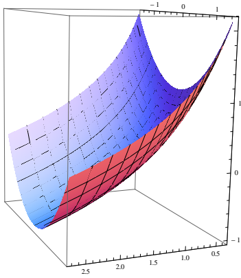
FIGURE 3. The domain \mathcal{B}^3
