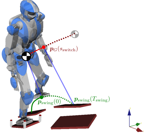
Fig. 3. Preview of swing-foot (green) and COM (light and dark red) trajectories during a single-support phase. Retiming the swing foot path under conservative constraints yields a swing duration T_{\text{swing}} . This value is then converted into retiming constraints on the COM trajectory, so that TOPP uses the single-support CWC up to \mathbf{p}_G(s_1) (light red) and the double-support one afterwards (dark red).
