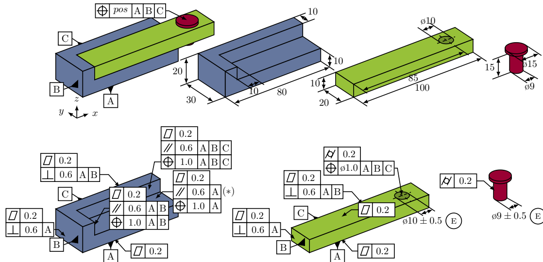
Fig. 2. Case Study: Functional Key Characteristic of the Assembly (top left), Part Measures (top right), and specified Geometric Tolerances (bottom).
