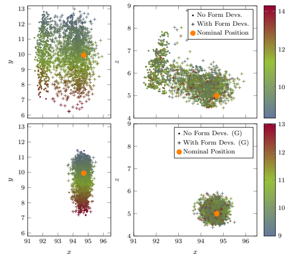
Fig. 11. Coordinates of a selected Node on the bottom of the Pin in the global coordinate system (see Fig. 2). Top shows the Results of the Worst-Case and bottom of the Statistical Tolerance Analysis, Colours indicate the Position Deviation pos of the respective Sample.
