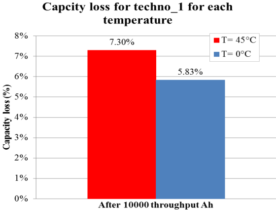
Figure 9 : Cycling in a range of SoC first results: Capacity loss after the first 10000 throughput Ah
