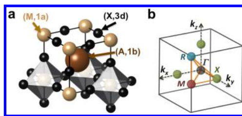
Figure 1. (a) Real space 3D view of the Pm-3m reference cubic crystal structure of metal–halide AIP or HOP of general formulas \text{AMX}_3 where A is an inorganic or an organic cation such as \text{CH}_3\text{NH}_3^+ , M a metal, and X an halogen. In HOP, the \text{CH}_3\text{NH}_3^+ cation is located at the center of the cube with an averaged position sketched by the brown ball. (b) Reciprocal space 3D view showing the first Brillouin zone (BZ) of the Pm-3m space group. Points of high symmetry in the cubic BZ are indicated by conventional letters: \Gamma denotes the origin of the BZ; X is the center of a square face at the BZ boundary; M (\frac{1}{2}, \frac{1}{2}, 0) is a center of a cube edge and R (\frac{1}{2}, \frac{1}{2}, \frac{1}{2}) corresponds to a vertex of the cube.
