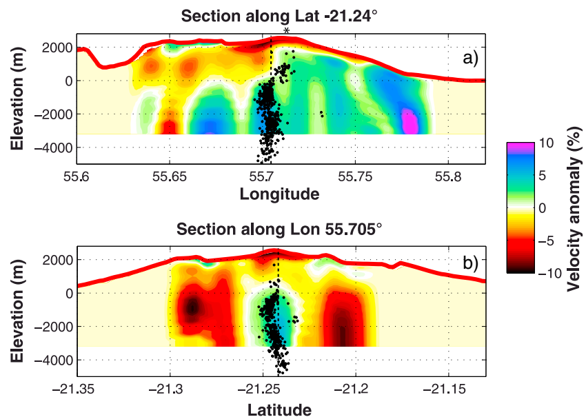
Figure 15. Vertical profiles through the isotropic Vs anomaly model. (a) EW profile at latitude -21.24^\circ . (b) NS profile at longitude 55.705^\circ . The thick red line is the local topography, and the black dots are the hypocenters from the 1998 intrusion [Battaglia et al., 2005]. The thick dashed black lines show the intersection with the other profile. Asterisk on the top frame shows the location of the summit crater.
