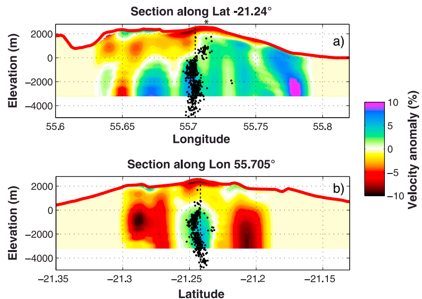
Figure 15. Vertical profiles through the isotropic V_s anomaly model. (a) EW profile at latitude -21.24^\circ . (b) NS profile at longitude 55.705^\circ . The thick red line is the local topography, and the black dots are the hypocenters from the 1998 intrusion [Battaglia et al., 2005]. The thick dashed black lines show the intersection with the other profile. Asterisk on the top frame shows the location of the summit crater.
