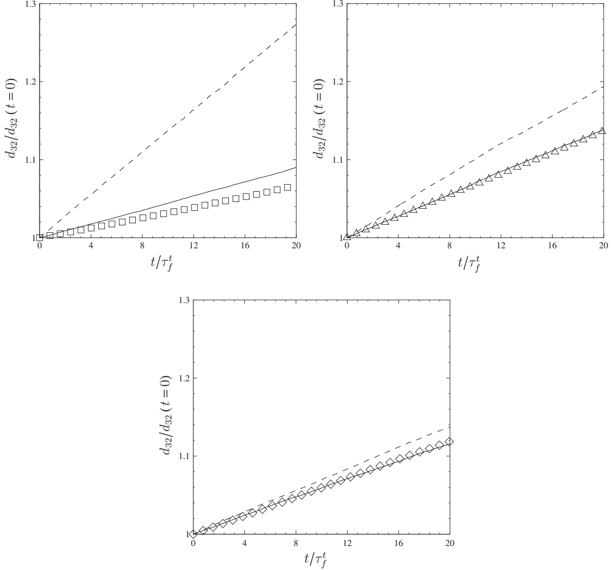
Fig. 24. Time-evolution of the Sauter diameter d_{32} = \langle d_p^3 \rangle / \langle d_p^2 \rangle of droplets suspended in THI. The symbols are the DPS/DNS, and lines are the stochastic simulations using Monte-Carlo algorithm (solid lines: CCV algorithm and dashed lines: standard algorithm).
