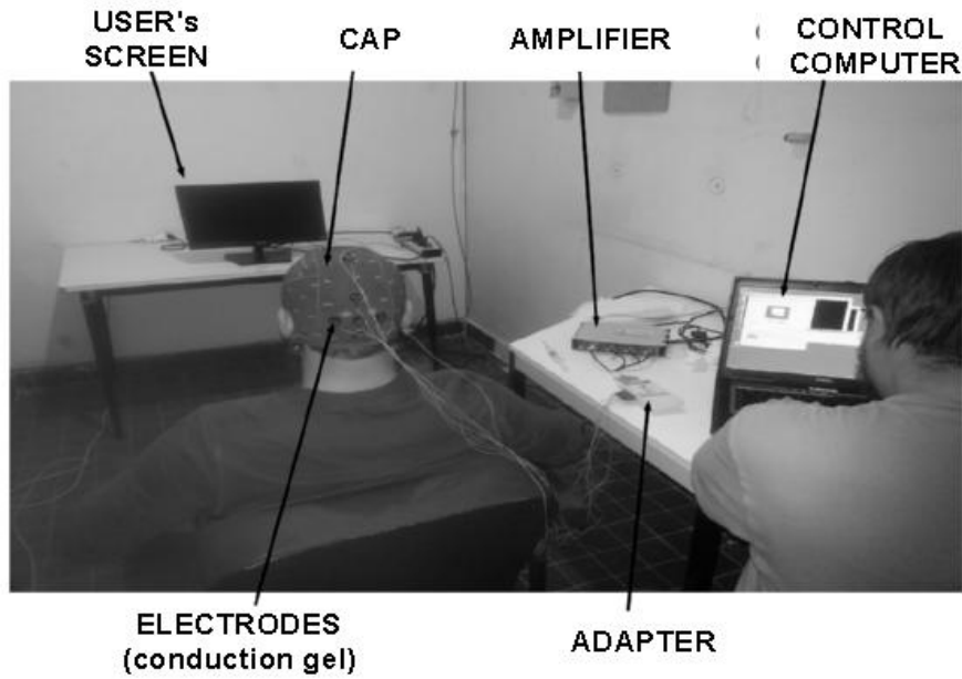
Figure 2: BCI experimental setup.
