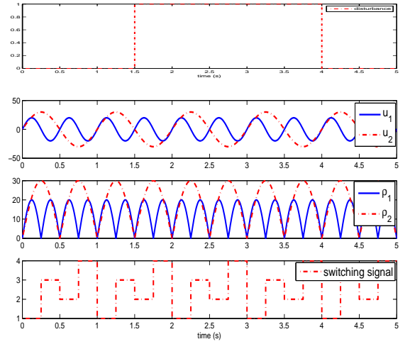
Fig. 8. Disturbance, control inputs, varying parameters, switching signal
