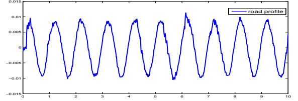
Fig. 3. Road profile
