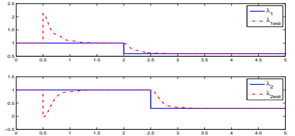
Fig. 9. The fault estimation result in a partial loss of effectiveness fault situation
