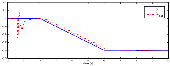
Fig. 7. A gradual damper fault scenario
