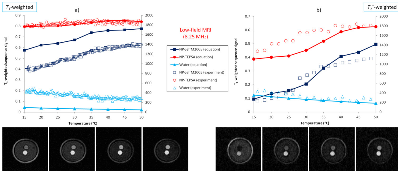
60 Fig. 7 Images taken on the low-field MRI scanner (8.25 MHz, 0.194 T) at increasing temperatures from 15 to 50°C with a) the T_1 -weighted sequence ( TR=100ms TE=2.8ms flip angle =70°) and b) the T_2^* -weighted sequence ( TR=300ms TE=12ms ), 160 \times 160 mm 2 field of view, 128 \times 128 matrix, 7 mm slice thickness. The external light grey circle was ascribed to a perfusion MRI contrast of the water circulating in the double-wall of the glass chamber (diameter 50 mm) as compared to water at rest inside the chamber (dark grey). The tube at the upper position was filled with Jeffamine ® M-2005 grafted USPIOs (1.1 mM Fe ) and the tube at the bottom position with the TEPSA-coated control (0.8 mM Fe ). The USPIOs exhibited a positive contrast (signal above the level of pure water) on all MR images except with the T_2^* -weighting (b) for the USPIOs grafted with the chains below their LCST (15-25°C). The open markers show experimental signals. The closed markers and the solid lines represent theoretical predictions using Eq. (5) with the experimental 65 values of T_1 , T_2^* , TE and TR . In the case of the Jeffamine ® M-2005 grafted USPIOs, a linear regression of the experimental signal (normalised to the initial value at 15°C) versus temperature leads to slopes of +1.9%/°C and +16.6%/°C respectively for the T_1 - and the T_2^* -weighted sequences, with correlation coefficients R=0.98 and R=0.97 , respectively. MRI cross-sections at the bottom line illustrate the variations of the signal plotted on the curves.
