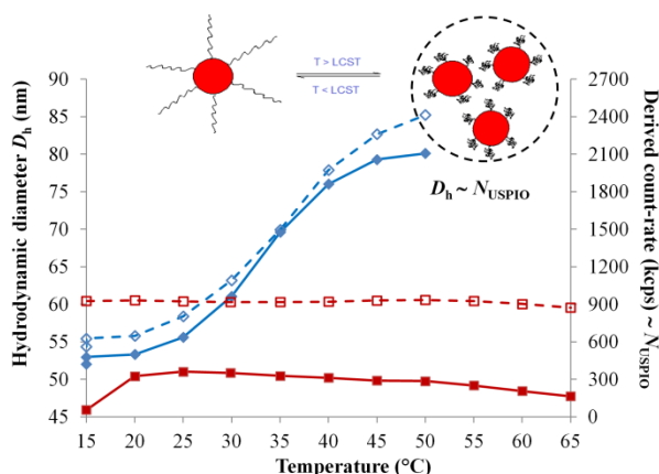
Fig. 4 Intensity-average hydrodynamic diameter D_h (nm, filled markers, solid lines) and derived count-rate in DLS (empty markers, dotted lines) vs. temperature for USPIOs grafted with Jeffamine ® M-2005 (blue) and M-2070 (red). The measurements were performed at 1 mM Fe in water.
