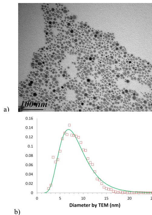
Fig. 2 a) TEM image of Jeffamine ® M-2005 coated-USPIOs (scale bar 100 nm) and b) histogram of TEM diameters deduced by automatic particle counting (red square) on five images with a total number of 7950 nanoparticles, and fitted by a log-normal law (green line) of parameters d_0=8 nm and \sigma=0.4 .
