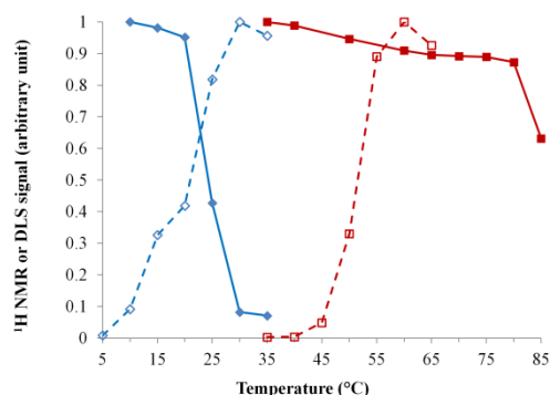
Fig. 1 Normalised area under the 1 H NMR spectrum (filled markers, solid lines) and derived count-rate in DLS (empty markers, dotted lines) vs. temperature for Jeffamine ® M-2005 (blue) and M-2070 (red) at 16 mg·mL -1 in H 2 O for DLS and 30 mg·mL -1 in D 2 O for NMR. The LCST is determined at the inflection points of both curves, 22 \pm 2^\circ\text{C} for M-2005, 52 \pm 2^\circ\text{C} for M-2070 (in that case a second transition above 80^\circ\text{C} is visible by NMR, corresponding to full dehydration of the chains).
