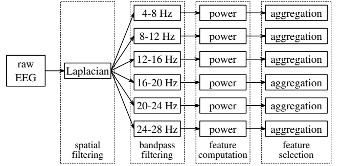
Figure 1: Processing pipeline for the training mode.
