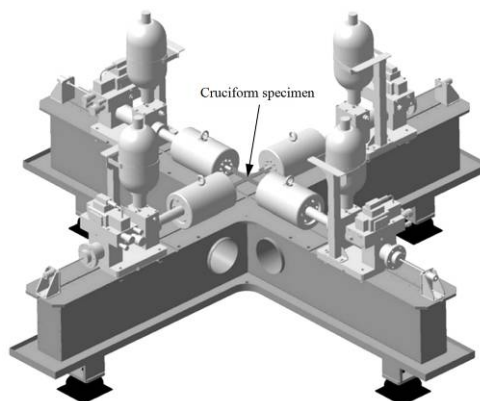
Figure 7. The in-plane biaxial tensile machine
