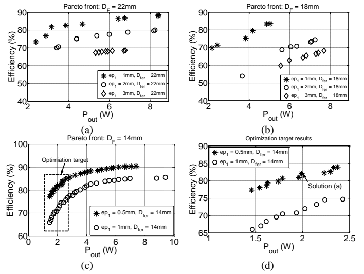
Fig.6 Pareto fronts' results of power supply function: (a) for D_F = 22mm , (b) for D_F = 18mm , (c) for D_F = 14mm , and (d) for our design target.
