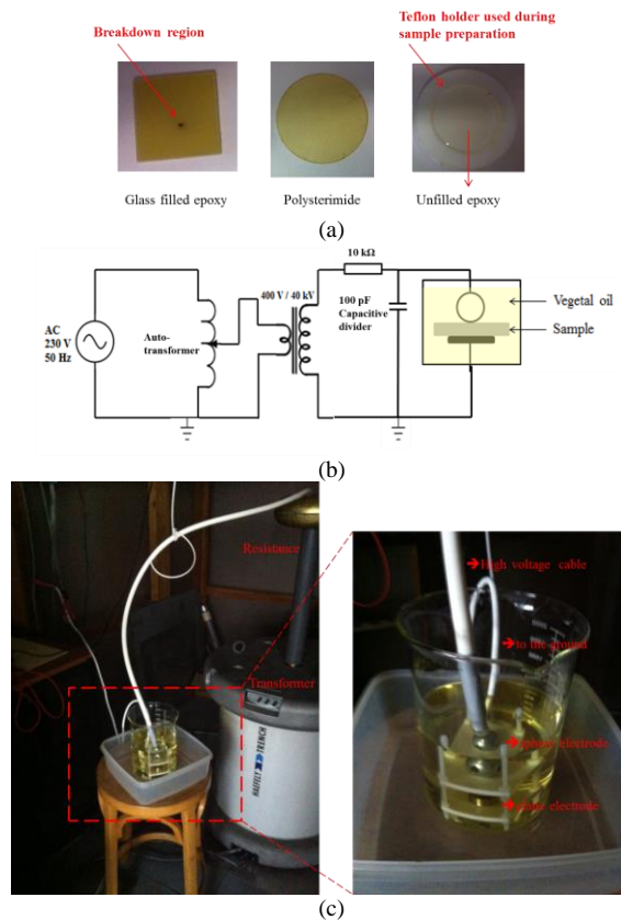
Fig. 2 Validation of the insulator breakdown voltages: (a) Sample insulator for testing experimental works: glass filled epoxy, polysterimide, (b) Schematic of the experimental set-up for breakdown measurement, (c) Experimental instruments for breakdown voltage measurement.
