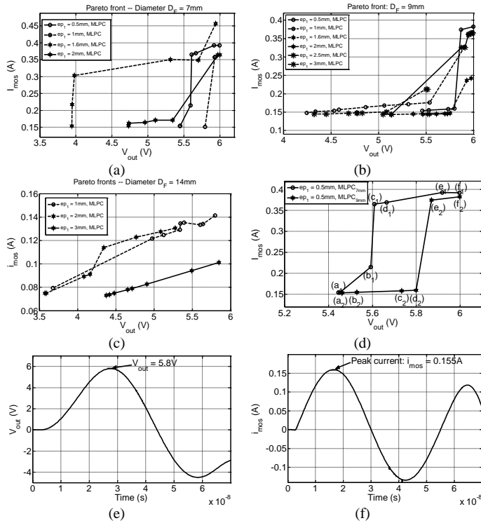
Fig.5 Pareto fronts' results: (a) for D_F = 7mm , (b) for D_F = 9mm , (c) for D_F = 14mm , (d) for our design target. (e) output voltage V_{out} waveform, and (f) primary side current waveform i_{mos} for solution ( d_2 )
