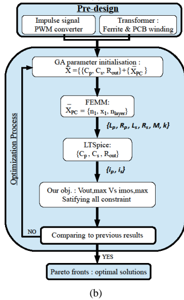
Fig.3 (a) Synopsis and schematic of the impulse transmission function based on a magnetic transformer. (b) GA flowchart for overall system optimization based on FEMM TM and LTSpice TM .
