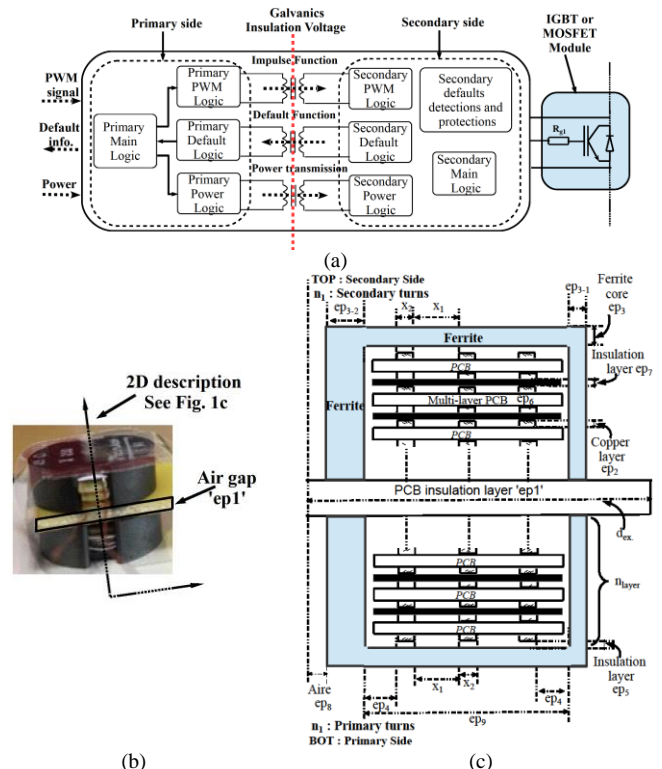
Fig.1 (a) Synopsis of a single channel gate driver. (b) a pot core ferrite planar transformer with winding on PCBs. (c) 2D descriptive of pot core planar transformer geometric.
