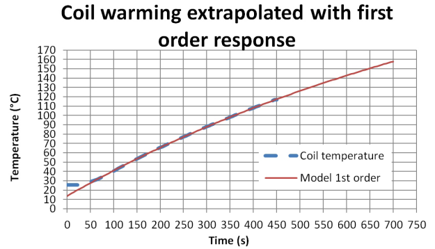
Fig. 9: MICA200M temperature on coil
