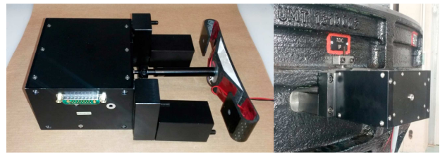
Fig. 2: MICA integrated in turning support
