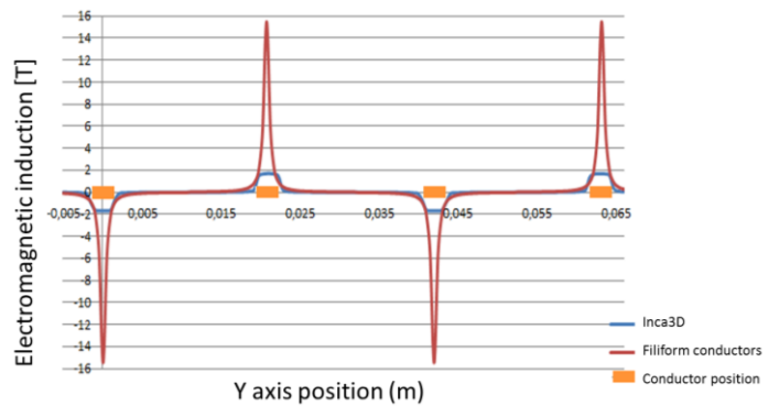
Fig. 7 Electromagnetic induction along x axis for y=0.
