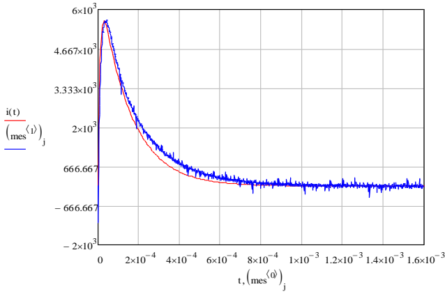
Fig. 12 Power supply current signal, from mathematical expression i(t) and from measurements mes^{<sup>t</sup>} .
