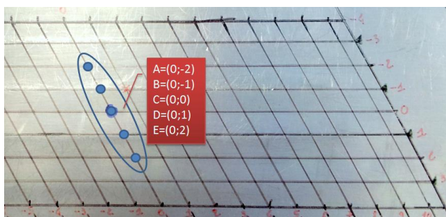
Fig.20 Evaluation points on the abrasion shield or plate [4].
