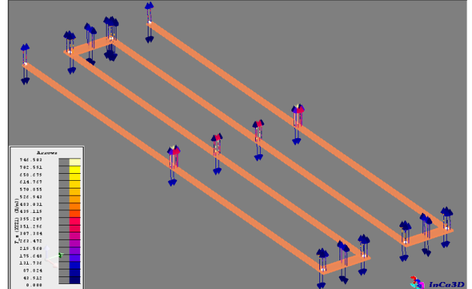
Fig. 6 Representation of Laplace force vectors, from InCa3D.
