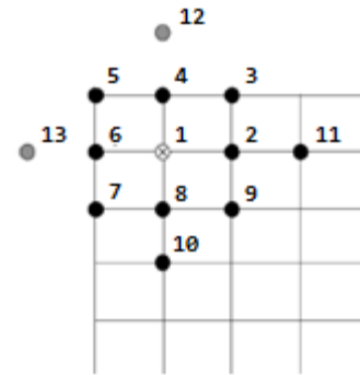
Fig. 16 Elements array for finite difference method.
