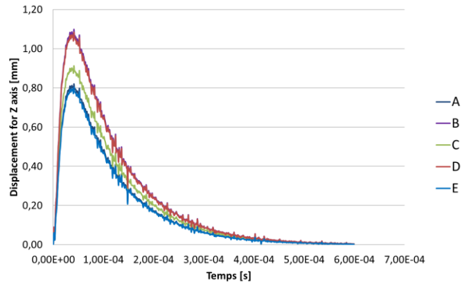
Fig. 21 Displacement results for static resolution.
