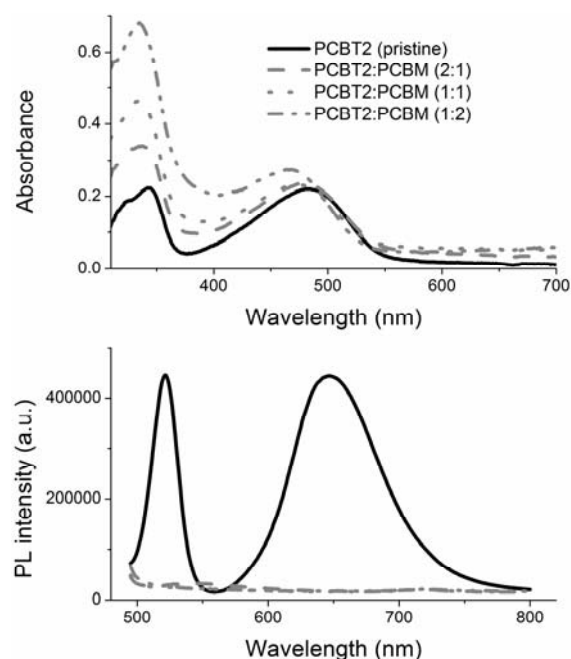
FIGURE 5. (a) Light absorption and (b) photoluminescence (excited at 481 nm) spectra of PCBT2:PCBM blends at different ratios in solid state.
