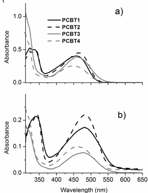
FIGURE 3b). This might be explained by a better conjugation along the 2,7-PCBTs chain. 55 Indeed, the 3,6-PCBTs induce conjugation breaks on the nitrogen atom, which limits the conjugation length and thus lower the absorption wavelengths. 46
