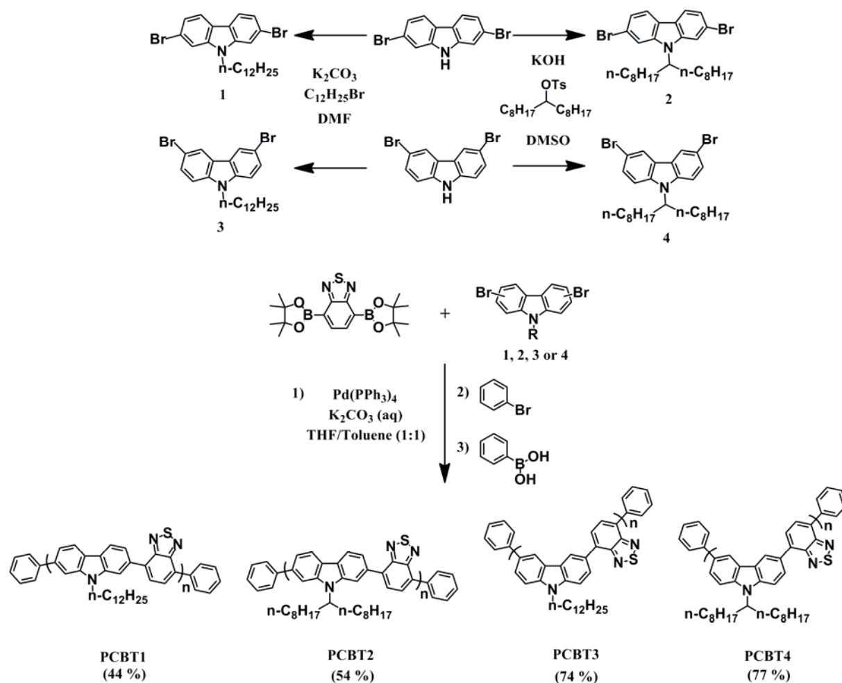
SCHEME 1 Synthesis of carbazole monomers and subsequent PCBTs by Suzuki cross-coupling. dibromocarbazoles were obtained in good yields (47-77 %). Their chemical structures were confirmed by ^1\text{H} (FIGURE 1), ^{13}\text{C} and ^1\text{H} - ^{13}\text{C} HSQC NMR, as well as FTIR and HRMS (see experimental section and supporting information, figures S2 to S9, for details ).
