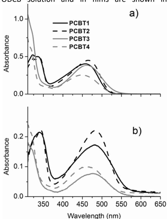
FIGURE 3. As frequently observed for alternated copolymers, all prepared PCBTs showed two broad absorption bands in the range of 300-350 nm and 440-500 nm in both solution and film states. 52 On the one hand, the high-wavelength band corresponds to the intramolecular charge transfer (ICT) from the electron-rich subunit (carbazole) to the electron-deficient one
