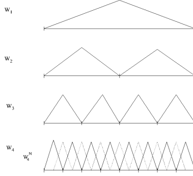
Figure 3.6: One dimensional W_{\underline{l}}^{(L)} spaces: W_1^{(L)} , W_2^{(L)} , W_3^{(L)} , W_4^{(L)} and the nodal representation W_4^{(L,N)}
