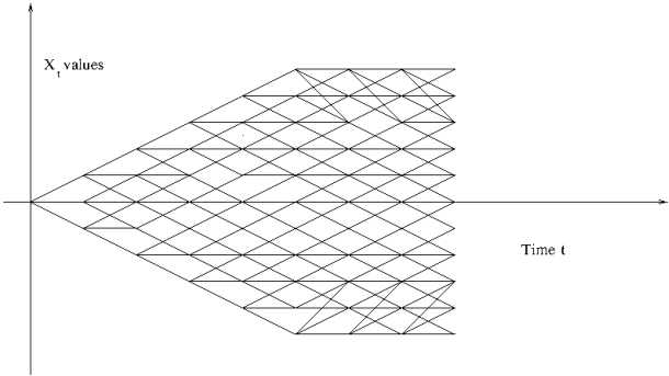
Figure 5.1: Trinomial tree
