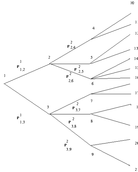
Figure 5.2: Non-recombining tree
