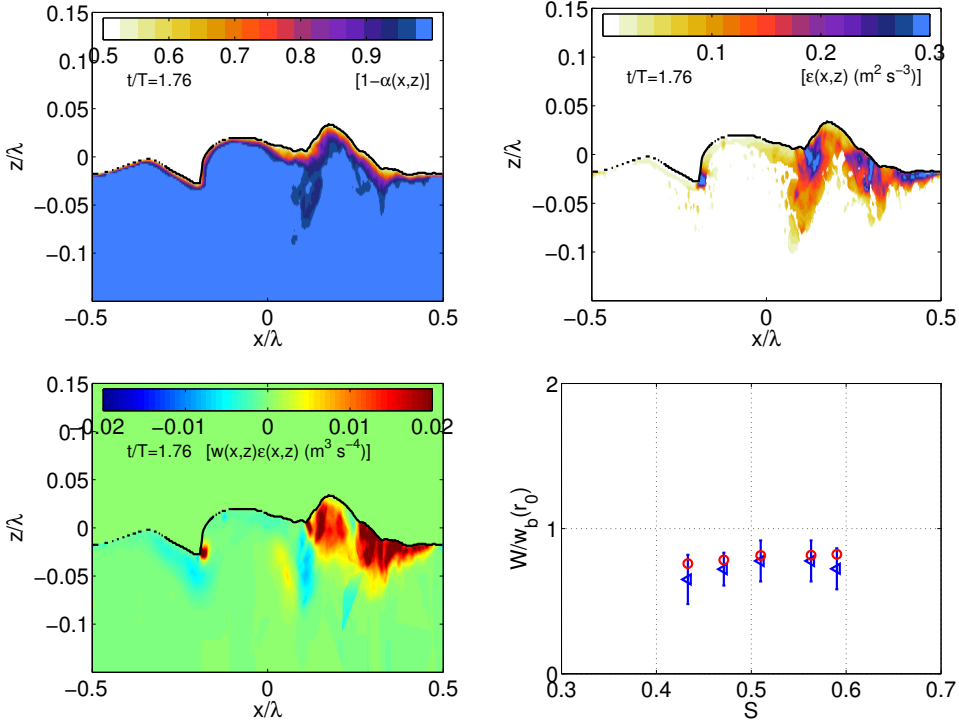
Figure 11: Example of transversally-averaged maps (in the water) of (a) [1 - \alpha(x, z, t)] , (b) \varepsilon(x, z, t) , and (c) w(x, z, t)\varepsilon(x, z, t) at t/T = 1.76 as a function of x and z , for S = 0.55 . These are used to calculate the weighted velocity W = \int w(x, z, t)\varepsilon(x, z, t)dtdxdz / (\int \varepsilon(x, z)(1 - \alpha(x, z, t))dtdxdz) (Eq. 4.12). (d) Weighted velocity as a function of the initial wave slope, normalized by w_b(r_0 = 1\text{mm}) the rise velocity in clean water of a bubble of radius r_0 = 1\text{mm} . ( \triangleleft ): direct calculation of W from Eq. 4.12. ( \circ ): \bar{w}_b = w_b(\bar{r}) , the rise velocity in clean water from Eq. 3.8 of a bubble with a radius given by \bar{r} = \int r\bar{N}(r)dr / \int \bar{N}(r)dr .
