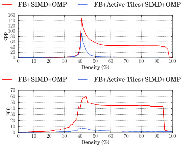
Figure 14. cfp for SIMD+OpenMP version with and without active tiles for KNC, for g = 1 (top) and g = 16
