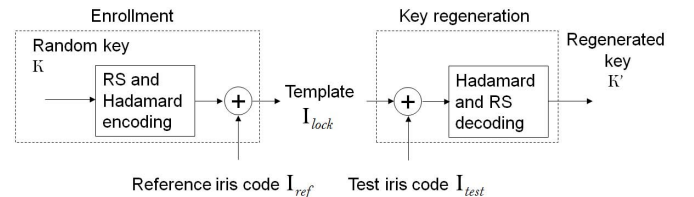
Fig. 1. Schematic diagram for biometric based cryptographic key regeneration system (similar to the Hao et al. [15] scheme).
