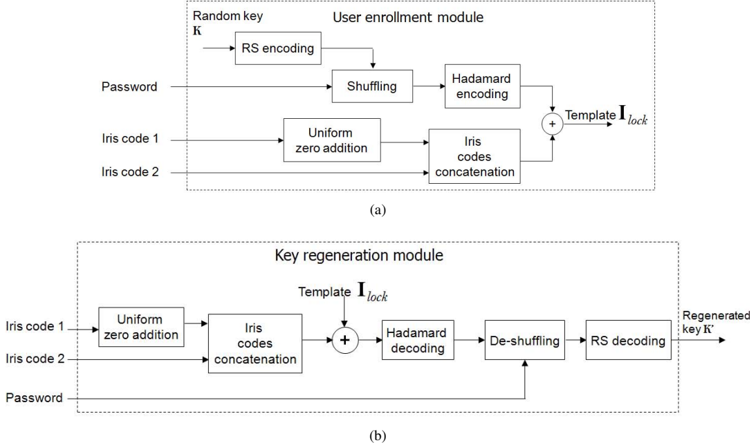
Fig. 2. Schematic diagram of the proposed multi-biometric based cryptographic key regeneration scheme using feature level fusion, weighted error correction, and password – (a) User enrollment phase; (b) Cryptographic key regeneration phase.
