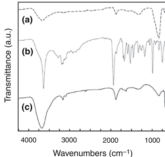
Fig. 1: FTIR spectra of: (a) Fe 3 O 4 , (b) IBA, and (c) IBA–Fe 3 O 4
