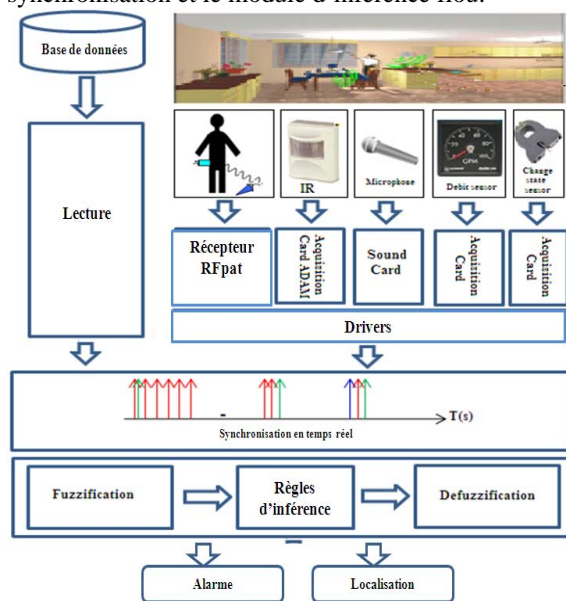
Figure 1: Architecture d'EMUTEM
