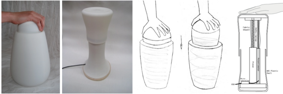
Figure 5: Left: the Spinotron affords vertical pumping and generates digitally synthesized sounds. Right: the configuration of the Spinotron device.
