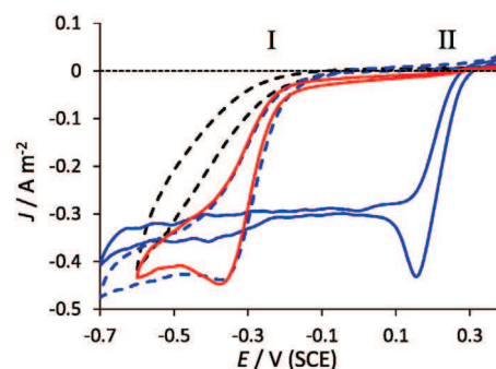
Fig. 2. Characterization of the biocathodes by cyclic voltammetry at 1 mV s ^{-1} . Red curve: CV of the biocathode formed under permanent forced aeration (reactors R1 and R2) at the end of experiment (day 21). Air flux was stopped just during CV recording. The two blue curves were recorded with the biocathodes formed in quiescent conditions (reactors R3 and R4) before (plain blue curve) and after (dotted blue curve) aeration had been applied for 24 h between days 20 and 21. Control voltammograms (black dotted line) were recorded at the beginning of the experiments before polarization started.
