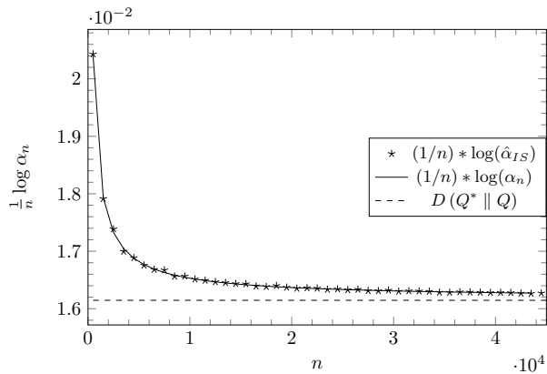
Figure 1. Values of \frac{1}{n} \log \hat{\alpha}_{IS} and of \frac{1}{n} \log \alpha_n compared to D(Q^* \| Q) .
