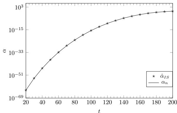
Figure 2. Values of \alpha_n and \hat{\alpha}_{IS} with respect to the threshold.
