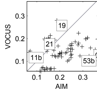
Figure 5: VOCUS vs AIM results for CC metric on VELER.
