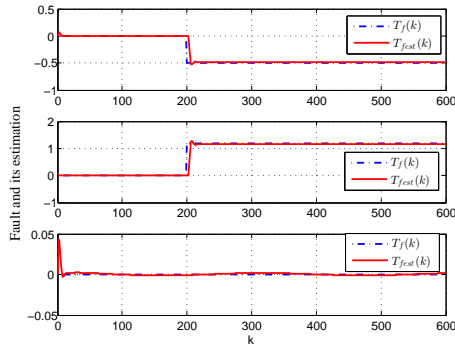
Fig. 2. Fault estimation result in an abrupt fault scenario
