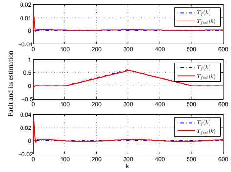
Fig. 4. Fault estimation result in a time-varying actuator fault scenario
