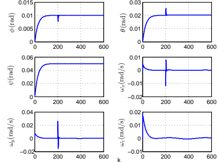
Fig. 1. Fault-tolerant control result in an abrupt actuator fault scenario
