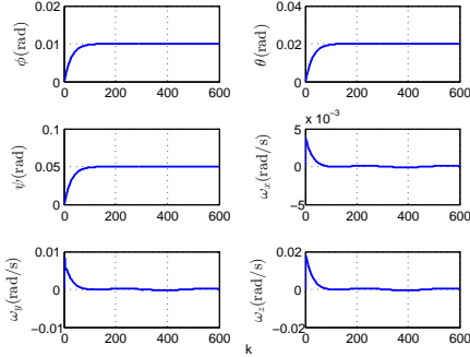
Fig. 3. Fault-tolerant control result in a time-varying actuator fault scenario
