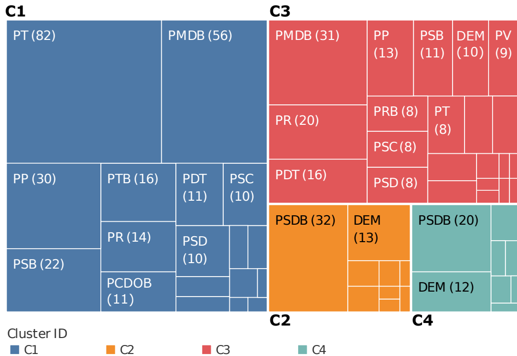
Figure 1: SRCC clustering results for the year of 2011, when solving version v1 of the voting network, by fixing the number of clusters in the solution to k = 4 .
