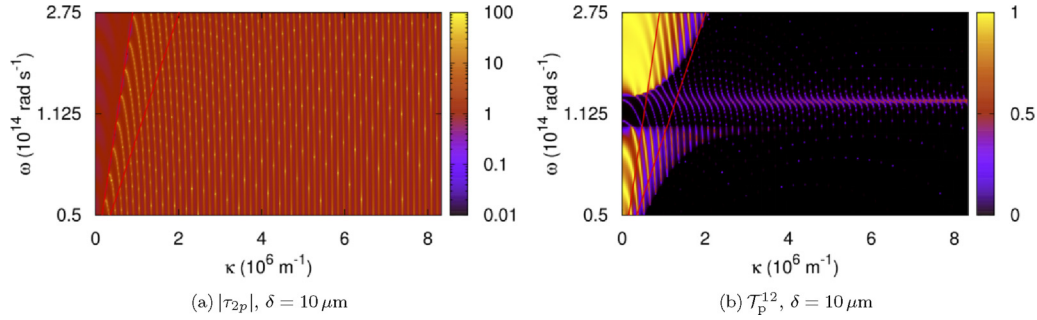
FIG. 7. Transmission coefficient of the intermediate slab |\tau_{2p}| and the energy transmission \mathcal{T}_p^{12} for p-polarized light for d = 100 nm and different thicknesses \delta of the intermediate hyperbolic slab of type I with \epsilon_x = \epsilon_\perp = 5 and \epsilon_z = \epsilon_\parallel = -1 in (\omega, \kappa) space. The inserted lines are the light line in vacuum ( \omega = c\kappa ) and the light line \omega = \sqrt{\epsilon_\parallel}c\kappa . As the reservoir we use again SiC.
