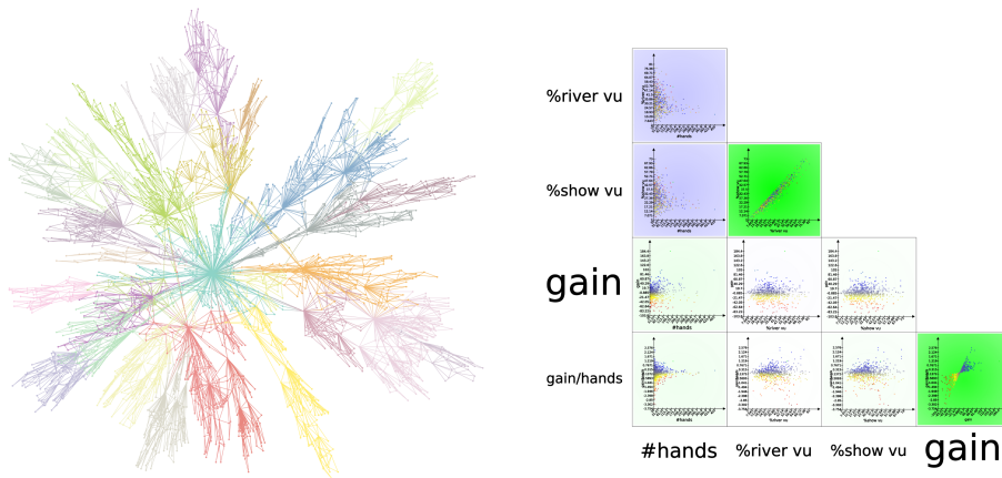
Figure 6: (Left) The node-link diagram view renders glyphs for nodes and curves for edges. The view provides navigation such as zoom and pan, bring and go [36], fish-eye views, and a magnifying glass. Direct editing of the graph elements and data, such as adding or removing nodes and edges or translating, rotating or scaling elements, is also supported. Other operations on this view include graph splatting, meta-node/graph hierarchy exploration, and texture-based animation. (Right) The scatter-plot 2D view renders attribute values to depict possible correlations between properties, and the matrix allows efficient navigation between dimensions. The view provides similar interaction to the node-link diagram and implements an interactor to search for correlation in an interactively defined subsets of elements. Splatting is also available in this view.
