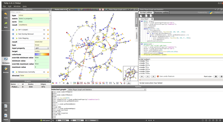
Figure 10: Python integration. The interactive console is shown at the bottom of the application and the Python view is displayed on the right. All the transformations performed using Python are applied in real time on the graph and can be visualized using another view (like the node-link diagram on the left).
