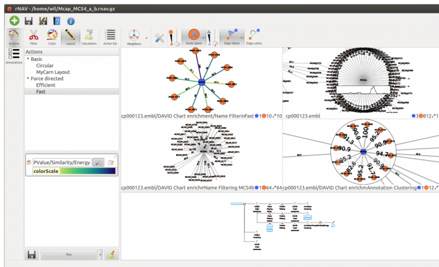
Figure 12: The rNAV software. The different views are linked and represent the same genomic data set, enriched (annotated) using DAVID, at different state of the analysis. The redundant annotations can be filtered and regrouped to ease the visual analysis and labels can be used to display several input information like p-value, similarity or interaction energy. Finally, the exploration tree view (bottom right) shows the steps taken to perform the analysis.
