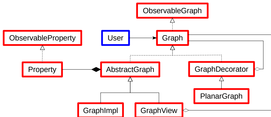
Figure 3: Overview of the meta-model class diagram. Instead of providing a complex set of classes, TULIP philosophy is to provide centralized access to the data structure through the Graph interface. The resulting implementation provides an optimized and extensible data structure.
