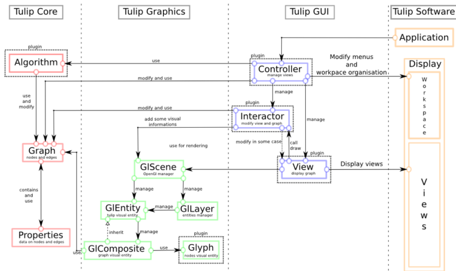
Figure 2: TULIP architecture overview. The TULIP framework consists of four packages. TULIP core provides an efficient data structures for relational data. TULIP graphics is a complete OpenGL rendering engine. TULIP GUI is a collection of widgets built on top of Qt library for the purpose of information visualization. Finally, TULIP software is an application for embedding algorithms, visualization techniques/interaction, and complete information visualization systems. All these packages can be dynamically extended through the plugin architecture of TULIP.
