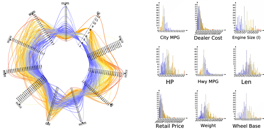
Figure 7: (Left) The parallel coordinates view depicts multivariate data, using the traditional parallel coordinates representation as well as a circular representation. In both views, lines can be rendered with smooth Bézier curves. Interaction with the view is supported through zoom and pan, axis edition/permutation/shifting, and multi-criteria/statistical selection. (Right) The histogram view provides a view of element frequency. A matrix of histograms allows for the visual comparison of several statistical properties of a set of dimensions. This view has a standard set of navigation and statistical interactors. Additionally, an interactor enables the user to build nonlinear mapping functions to any of the graph attributes such as size, colors, glyphs, etc.
