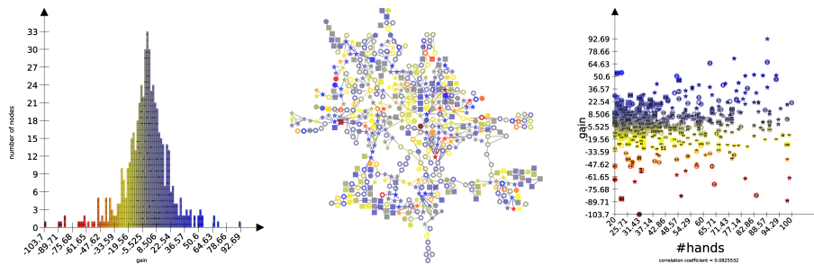
Figure 5: A centralized meta-model maintains coherence between views of a same graph. (Left) Histogram view. (Middle) Node-link diagram. (Right) Scatter-plot views. All three views share the same visual attributes (color, shape, size. . .) enabling the user to switch between views easily and keep track of selected elements from view to view.
