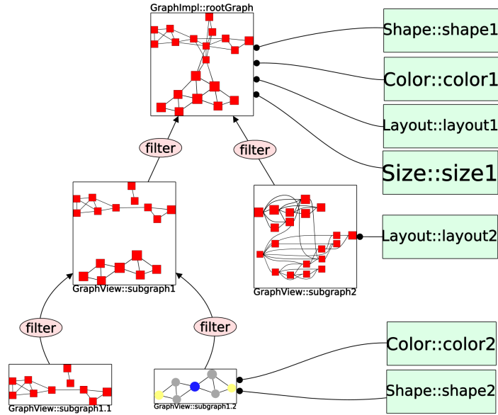
Figure 4: Graph Hierarchy (figure created with TULIP): TULIP provides management of a hierarchy of subgraphs through an efficient filtering mechanism of graphs. The inheritance mechanism of graph properties in the hierarchy maximizes the number of properties shared between subgraphs. For instance, Subgraph 1 inherits the layout of the root graph. The inheritance mechanism is also able to redefine properties in subgraphs like one would do in an object-oriented programming language. Subgraph 2, for example, has redefined its layout property but inherits the color, size and shape properties of its parent, whereas Subgraph 1.2 inherits its parent layout but uses different color and shape properties.
