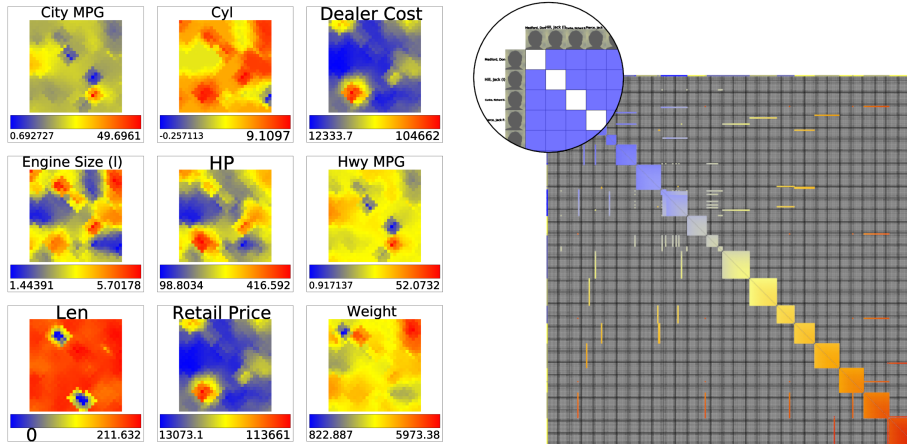
Figure 9: (Left) The self-organizing view implements Kohonen self-organizing maps [33]. Several kinds of topology/connectivity for the generated maps are supported as well as navigation and selection interactors. (Right) The matrix view implements a matrix view of the graph. This view has been built to support graphs with a large number of nodes and edges. Zooming and selection interactors are available for this view.
