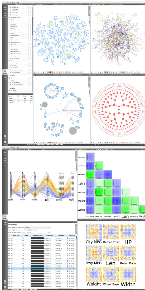
Figure 1: TULIP 4 is a framework that enables visualization researchers and application designers to operate on an algorithm, technique/interaction, and visual encoding level. The figure on the top shows an overview of TULIP with some graph drawing made with different algorithms and metrics. The figure on the bottom shows several views of the same data set with custom interactions. The data comes from [52] (cars data set).
