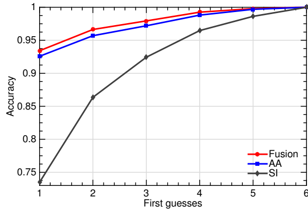
Fig. 3. Comparison of the overall CA between the 3 methods
