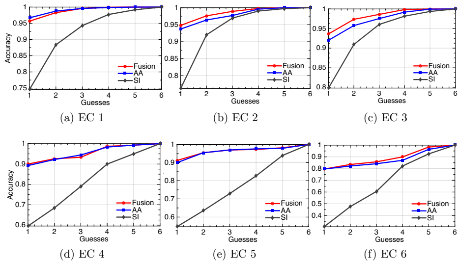
Fig. 4. Comparison of the CA for each true class between the 3 methods
