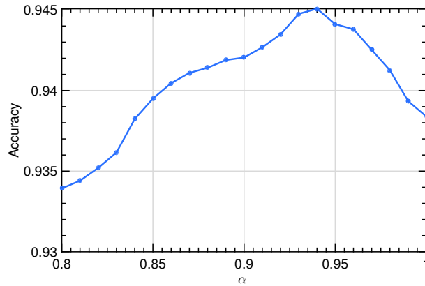
Fig. 2. Classification accuracy on the validation dataset as a function of the weight \alpha
