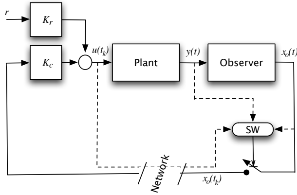
Figure 1: Observer based controller.
