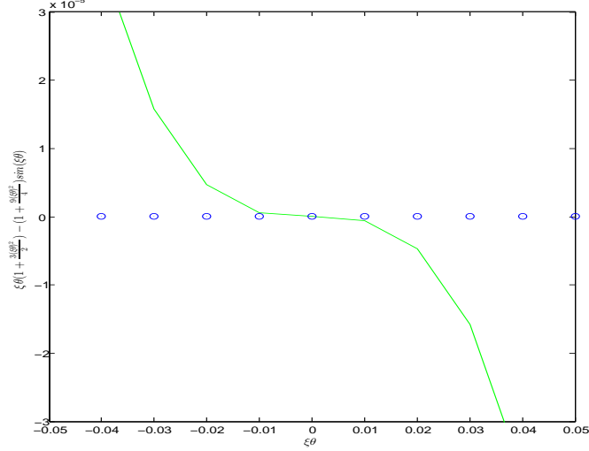
Figure 1: Graph of the function \xi \rightarrow \xi\Theta_\gamma \left(1 + \frac{3(\xi\Theta_\gamma)^2}{2}\right) - \left(1 + \frac{9(\xi\Theta_\gamma)^2}{4}\right) \sin(\xi\Theta_\gamma) over interval [-0.05, 0.05] . Also shown that zero is its singular point.
